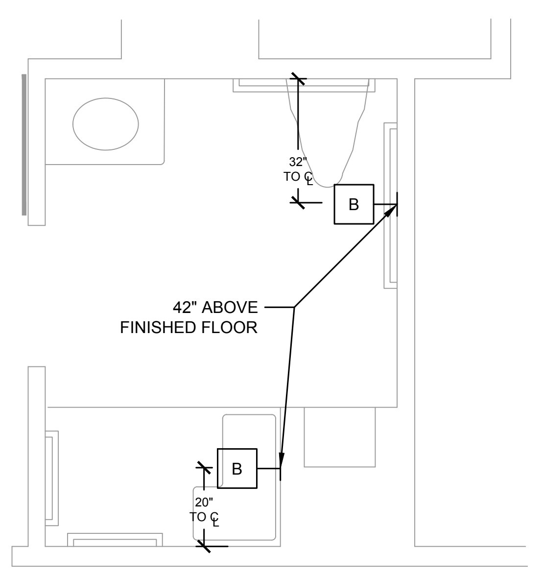
2 TYP. CONCIERGE TOILET ROOM FLOOR PLAN SCALE: NTS
