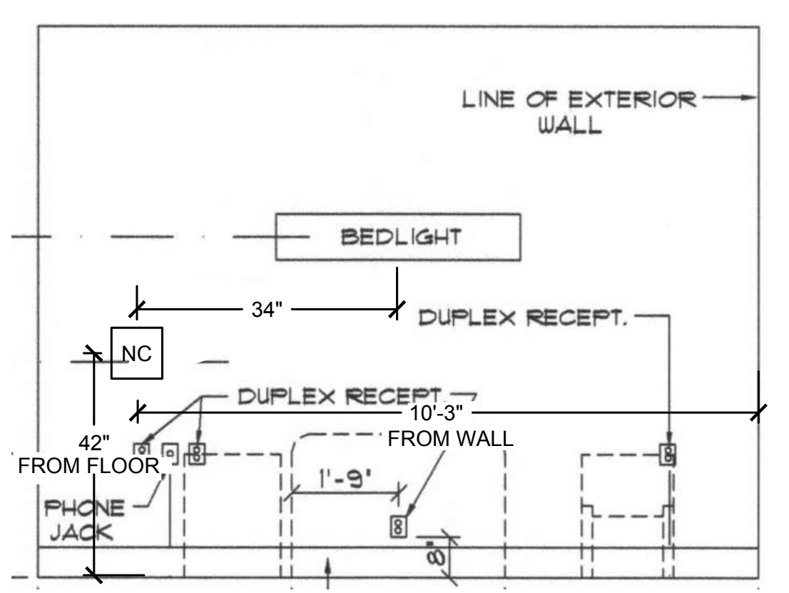
3 TYP. BEDWALL FOR TYP. BEDROOM SUITE SCALE: NTS
