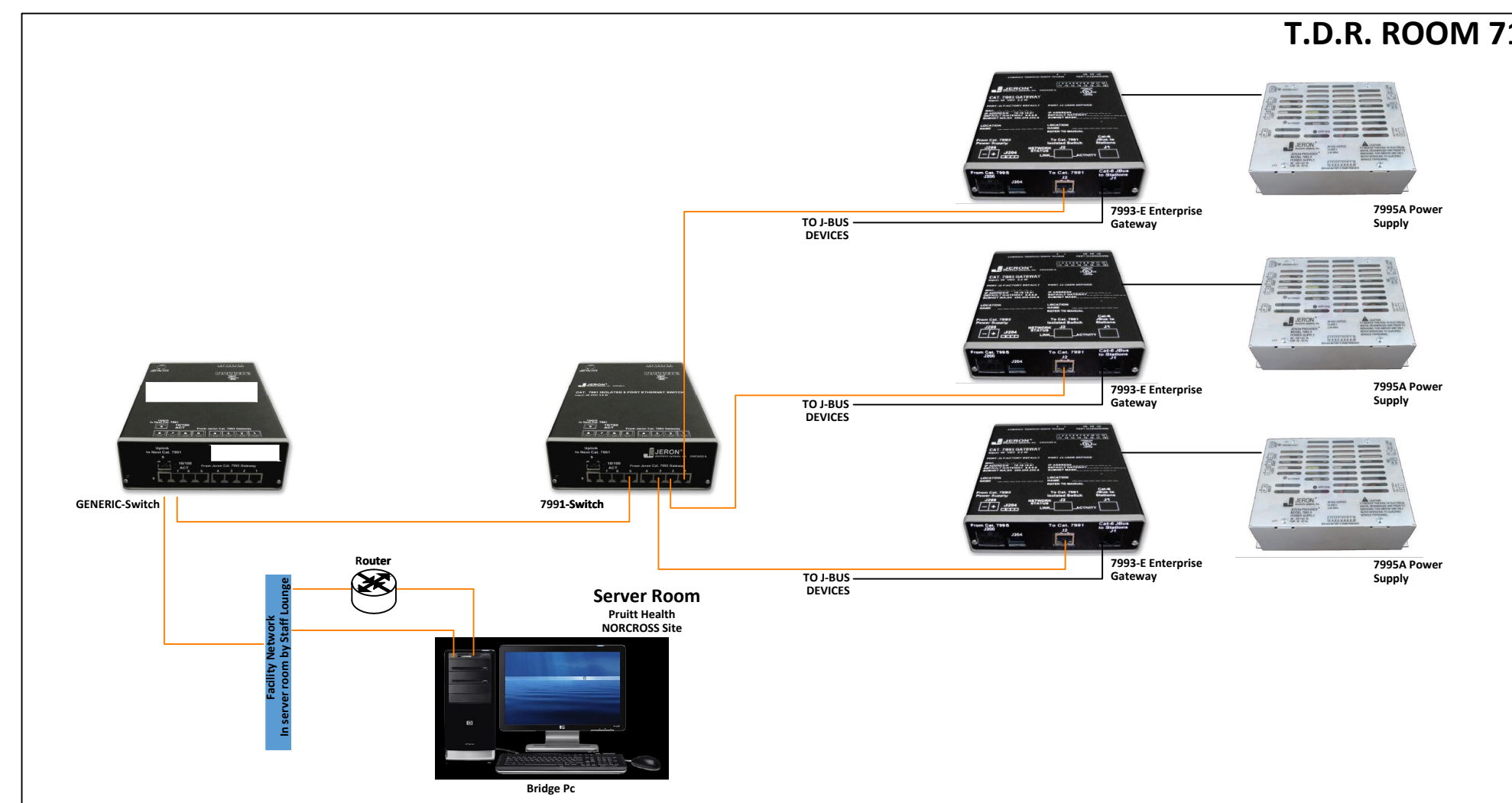
1 JERON IP NETWORK WIRING DIAGRAM SCALE: NTS
