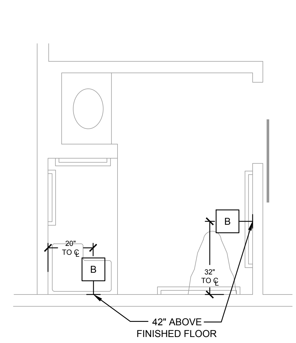
1 TYP. PATIENT TOILET ROOM FLOOR PLAN SCALE: NTS
