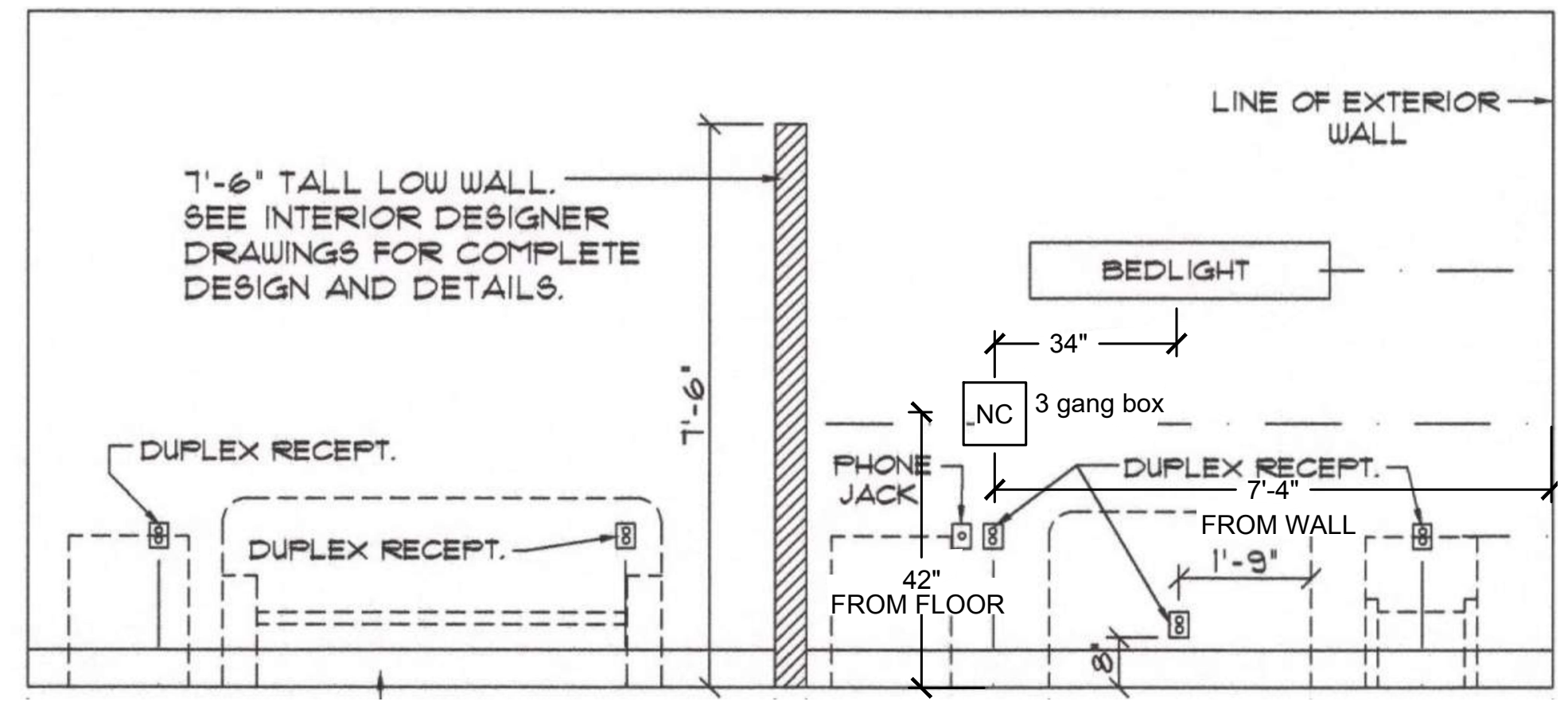
4 TYP. BEDWALL FOR TYP. CONCIERGE SUITE SCALE: NTS
