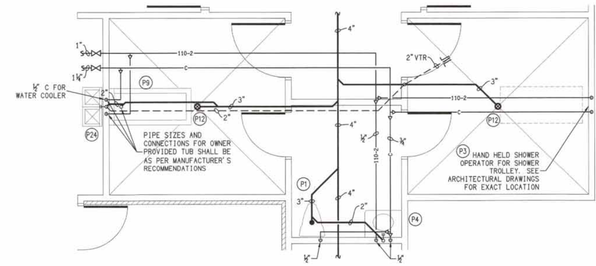
E ENLARGED PLUMBING PLAN P7 SCALE: 1/4" = 1'-0"
