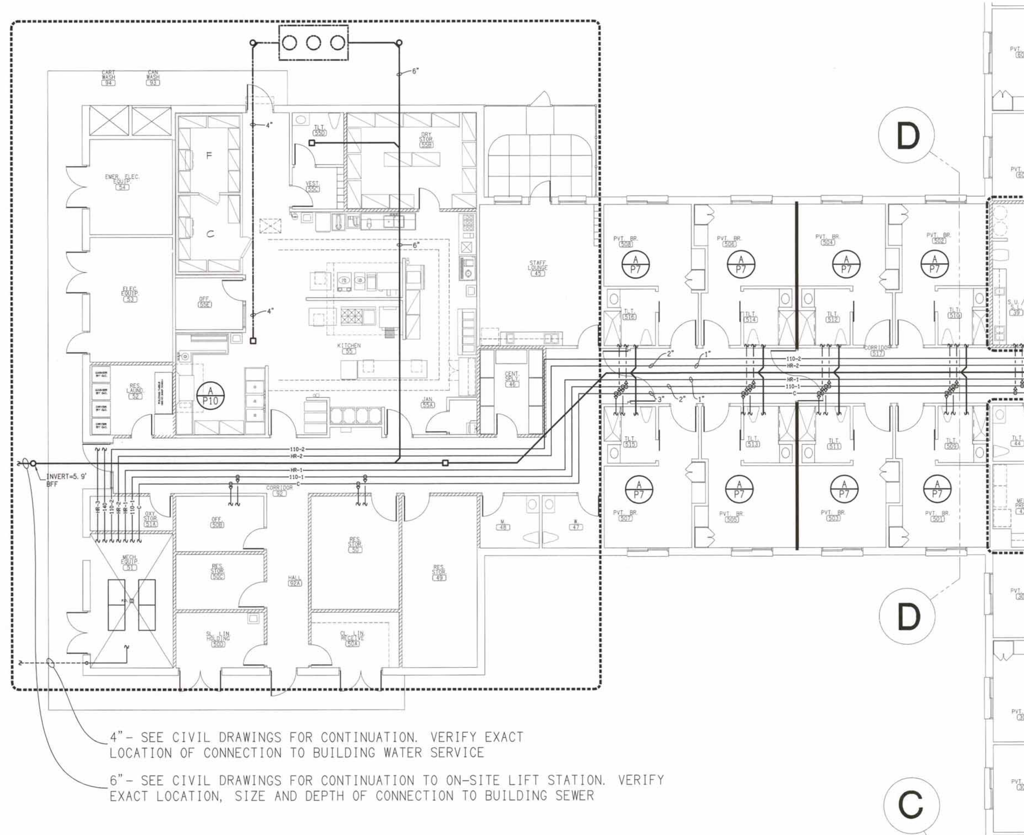
A PARTIAL PLUMBING PLAN P5 SCALE: 1/8" = 1'-0"
