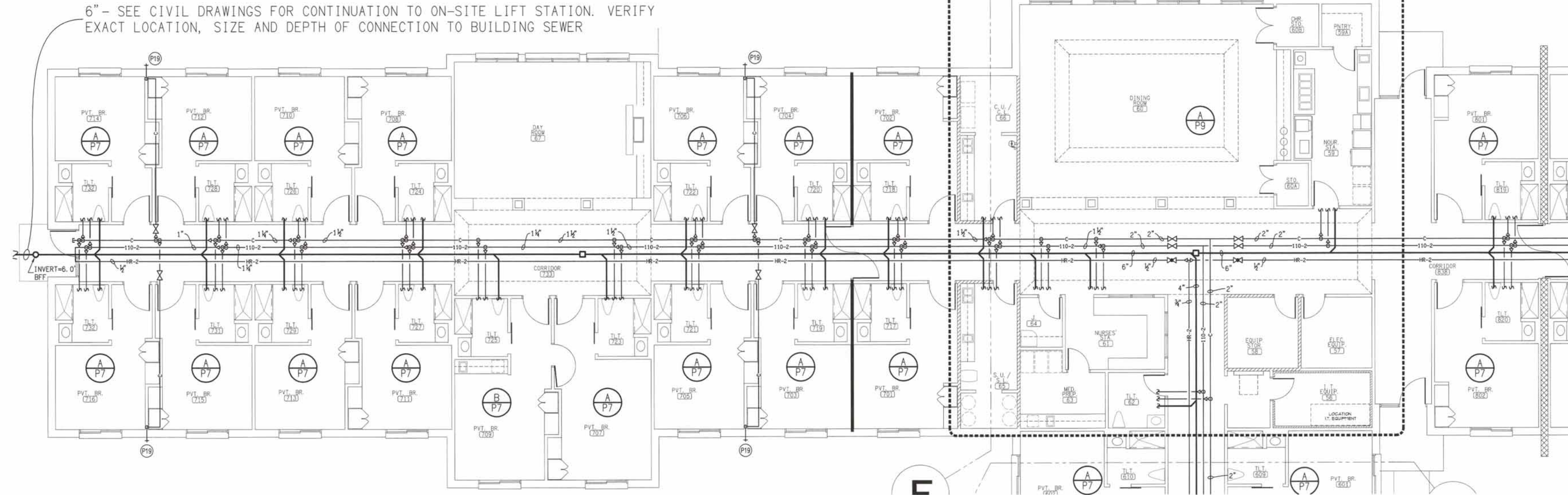
B PARTIAL PLUMBING PLAN P6 SCALE: 1/8" = 1'-0"
