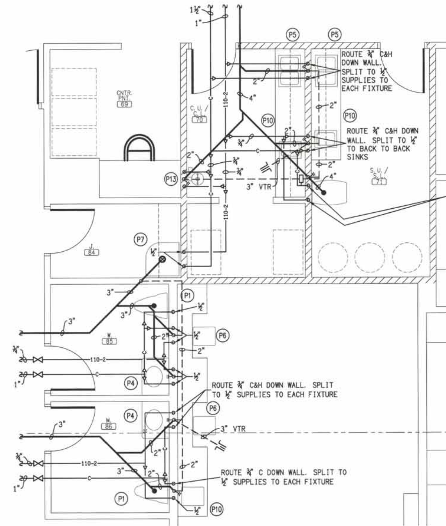
C ENLARGED PLUMBING PLAN P9 SCALE: 1/4\" = 1' - 0"
