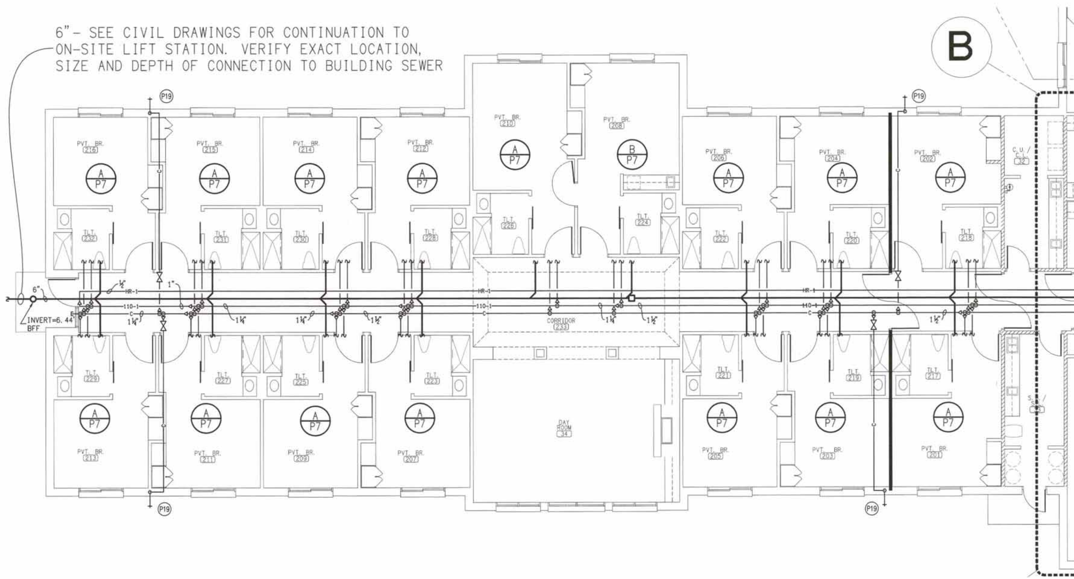
A PARTIAL PLUMBING PLAN P3 SCALE: 1/8" = 1'-0"
