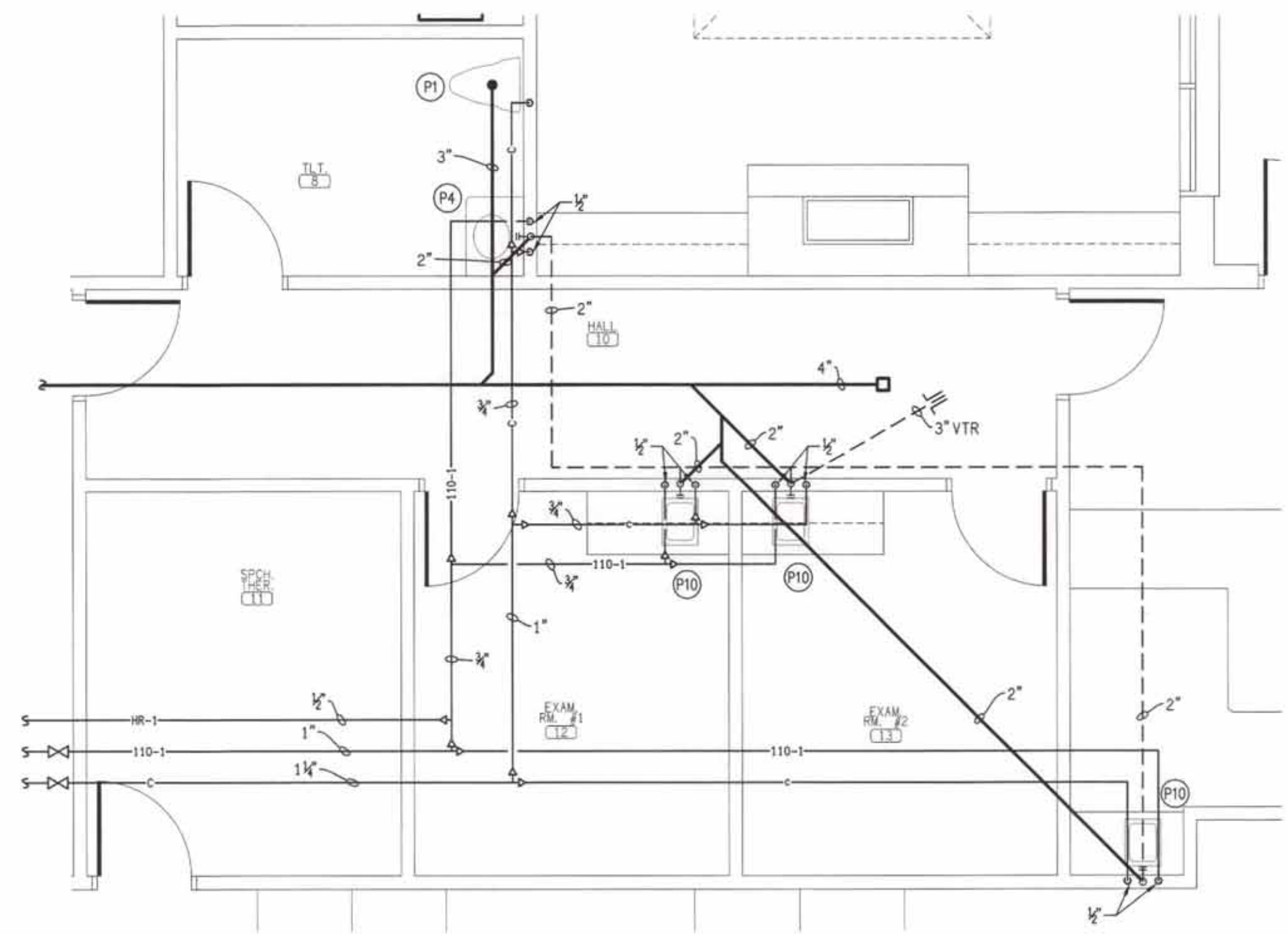
D ENLARGED PLUMBING PLAN P7 SCALE: 1/4" = 1'-0"
