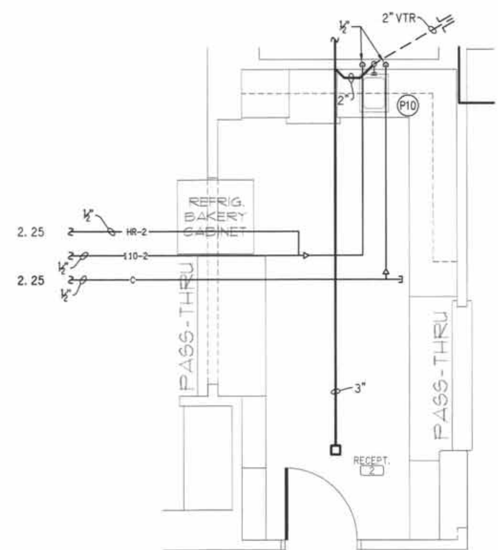
C ENLARGED PLUMBING PLAN P7 SCALE: 1/4" = 1'-0" RECEPTION
