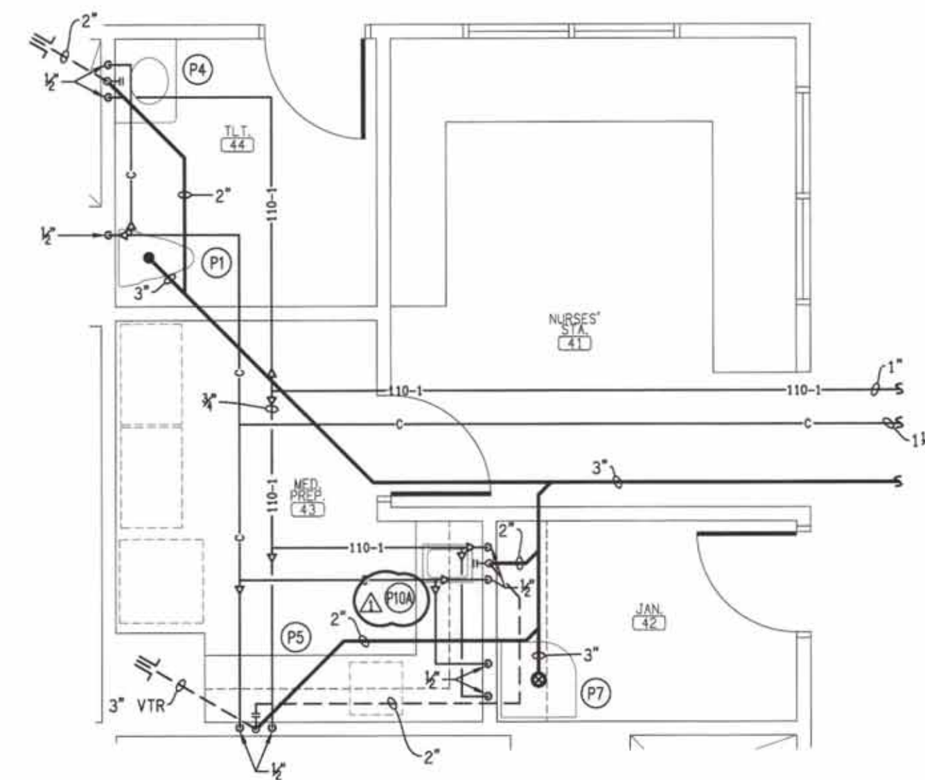
B ENLARGED PLUMBING PLAN SCALE: 1/4" = 1'-0" NURSE'S STATION
