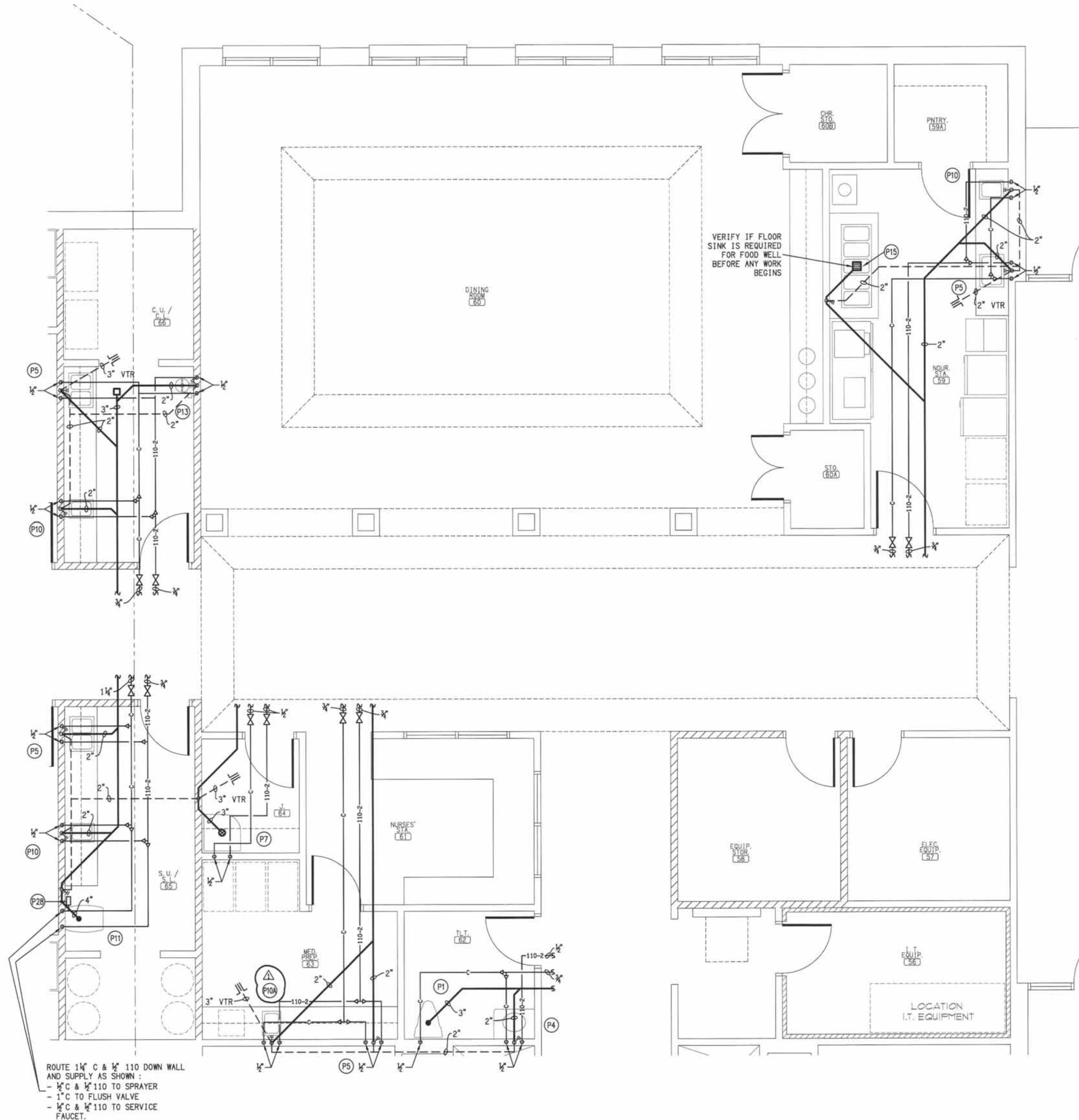
A ENLARGED PLUMBING PLAN P9 SCALE: 1/4\" = 1' - 0\" KITCHEN
