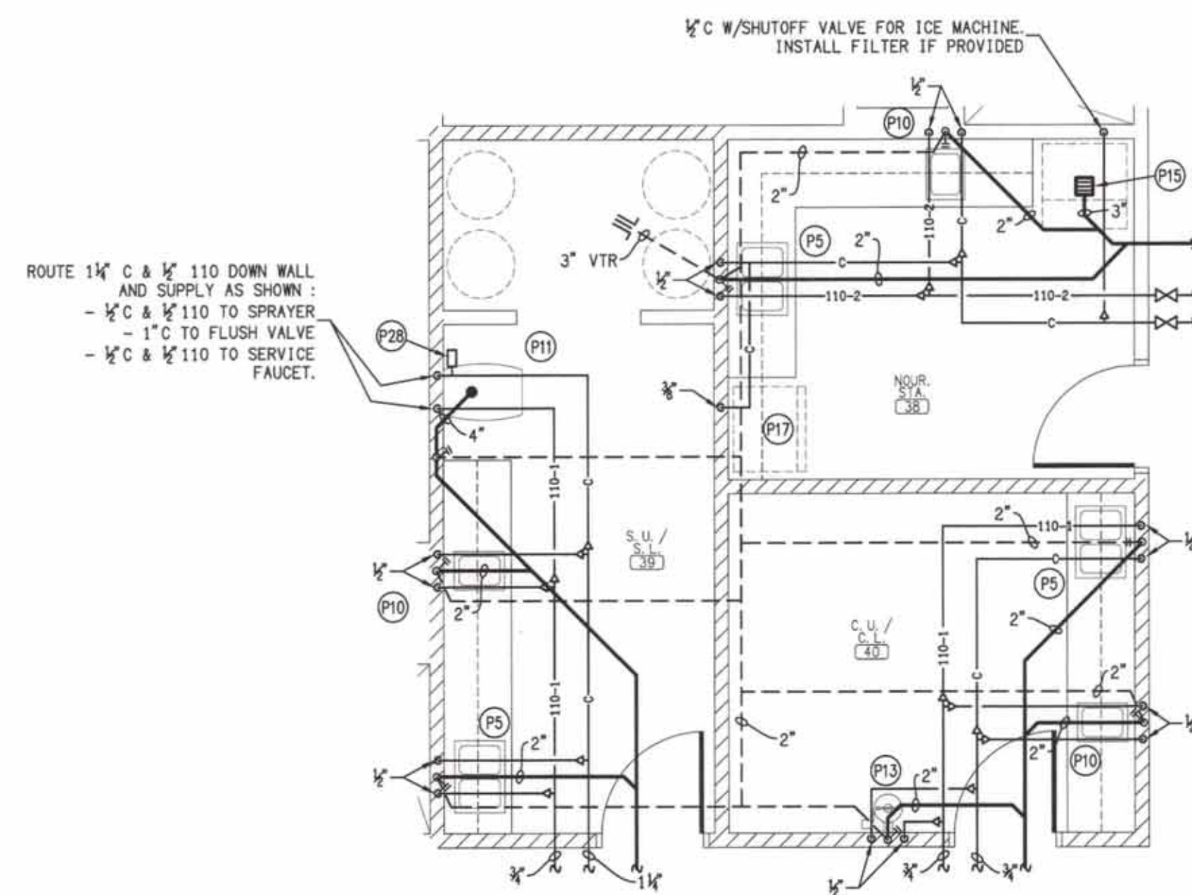
C ENLARGED PLUMBING PLAN SCALE: 1/4" = 1'-0"
