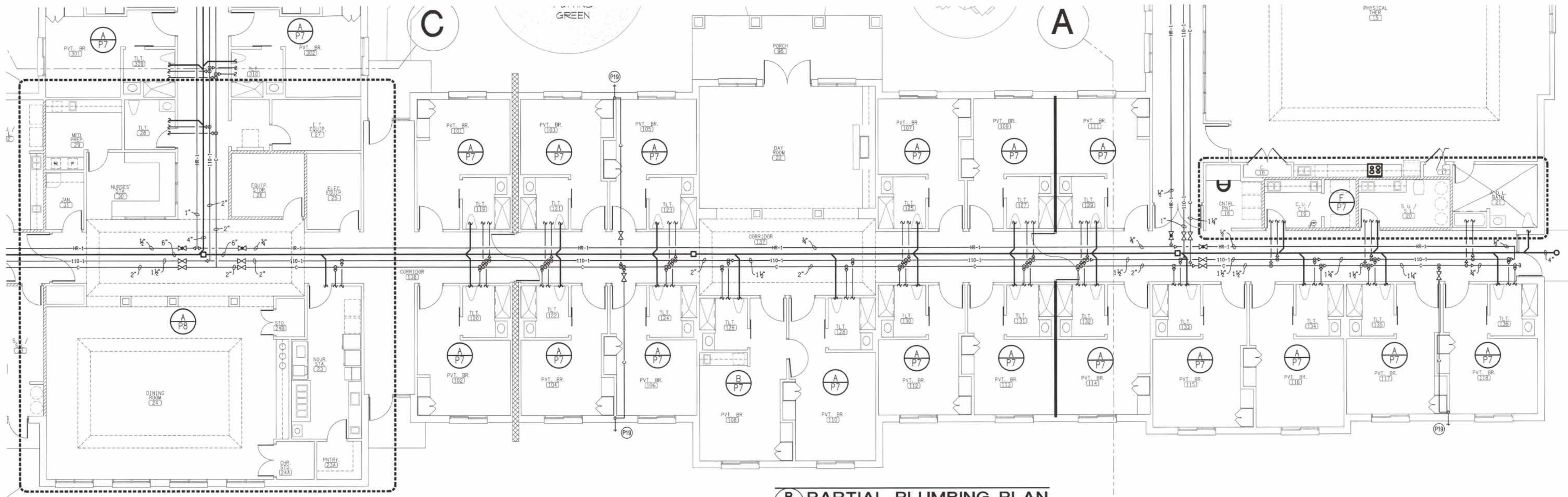
B PARTIAL PLUMBING PLAN P3 SCALE: 1/8" = 1'-0"
