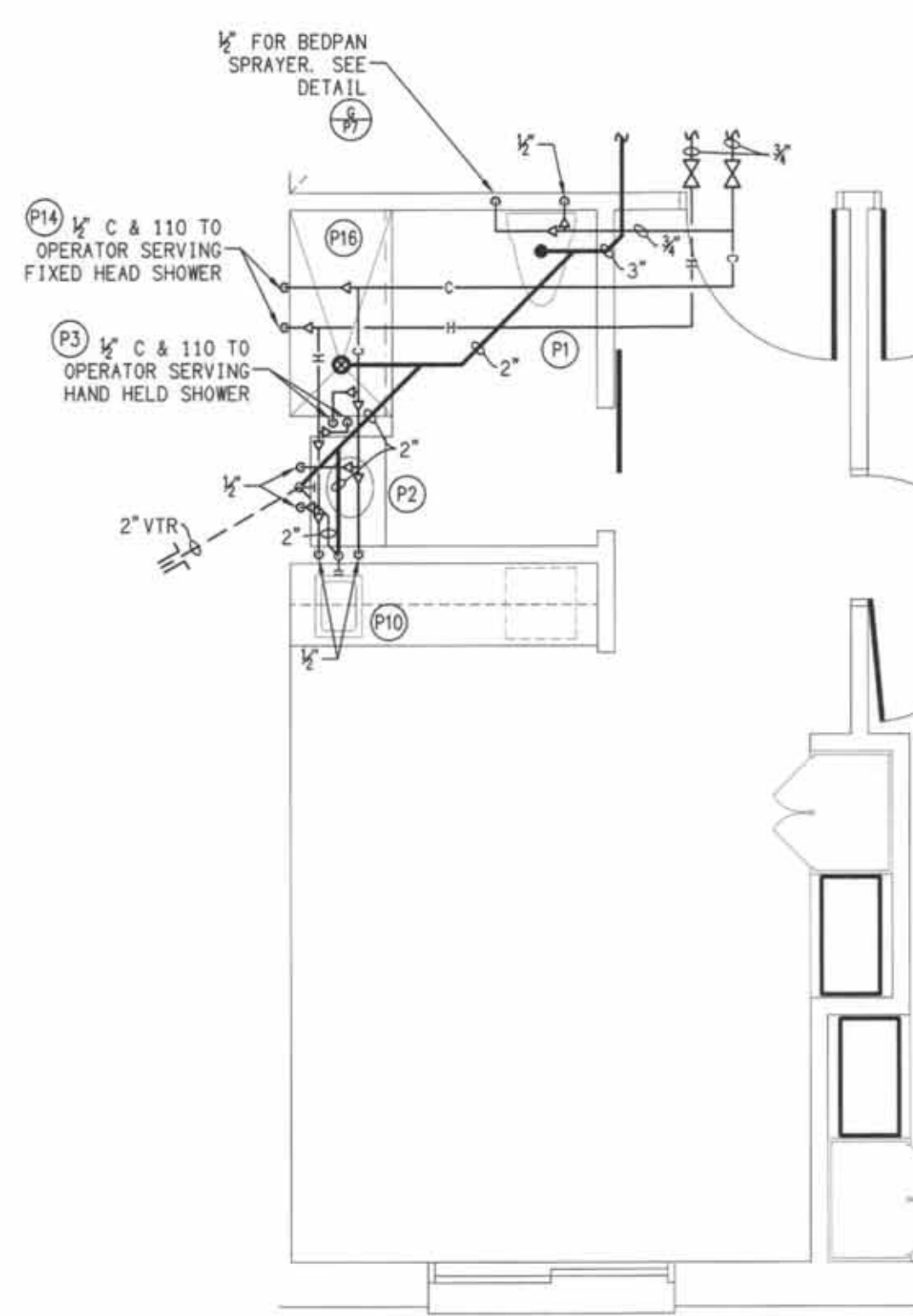
B ENLARGED PLUMBING PLAN P7 SCALE: 1/4" = 1'-0" TYPICAL ROOM
