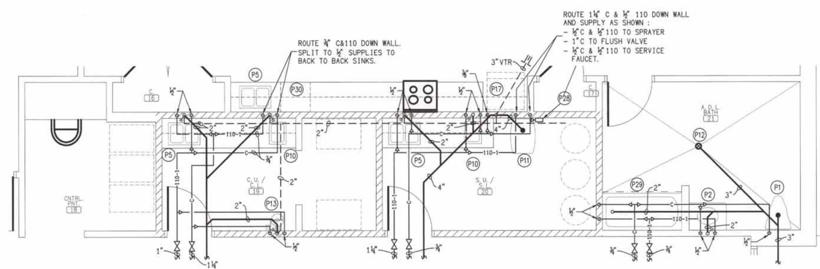
F ENLARGED PLUMBING PLAN P7 SCALE: 1/4" = 1'-0"
