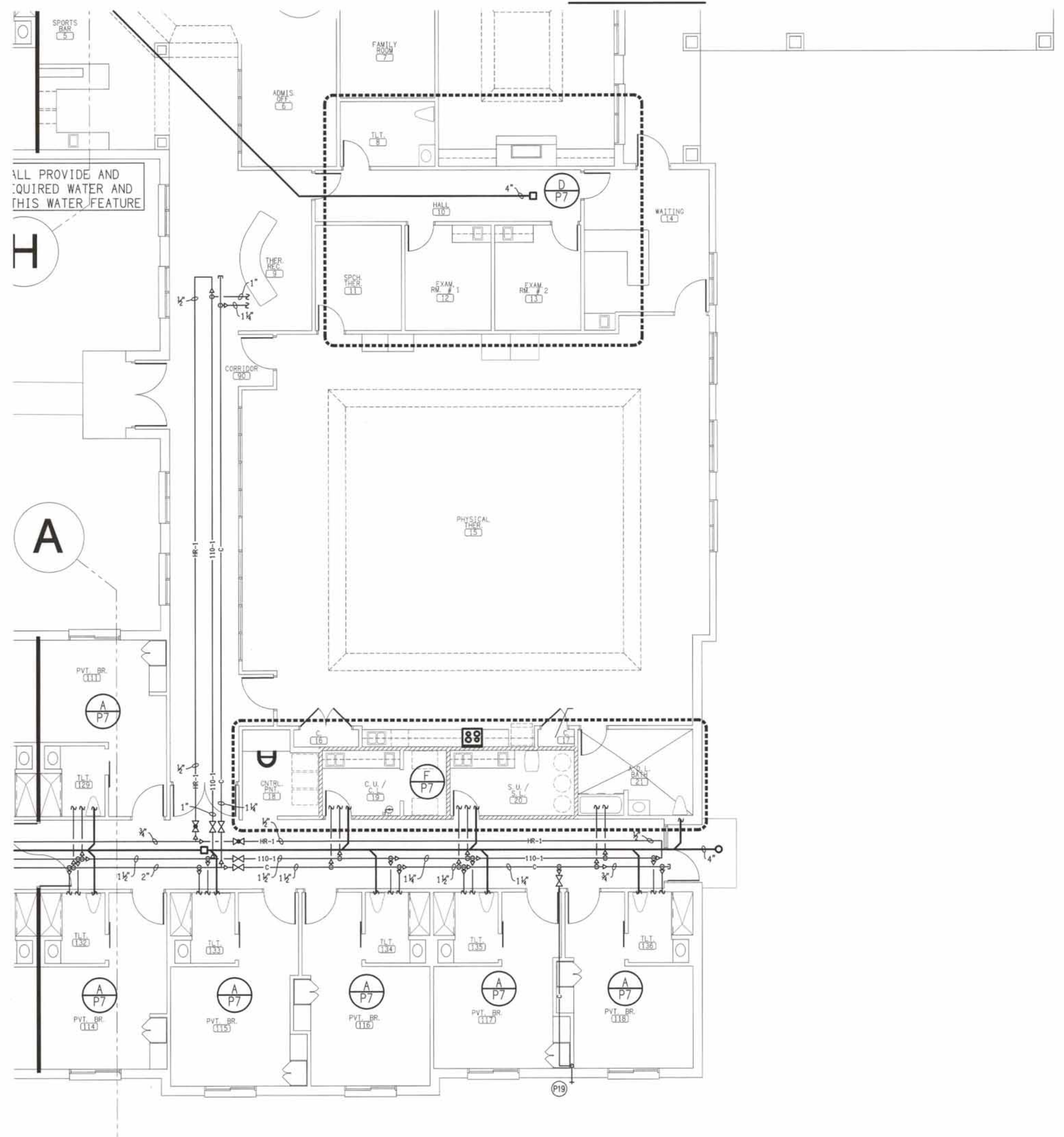
B PARTIAL PLUMBING PLAN P2 SCALE: 1/8" = 1'-0"
