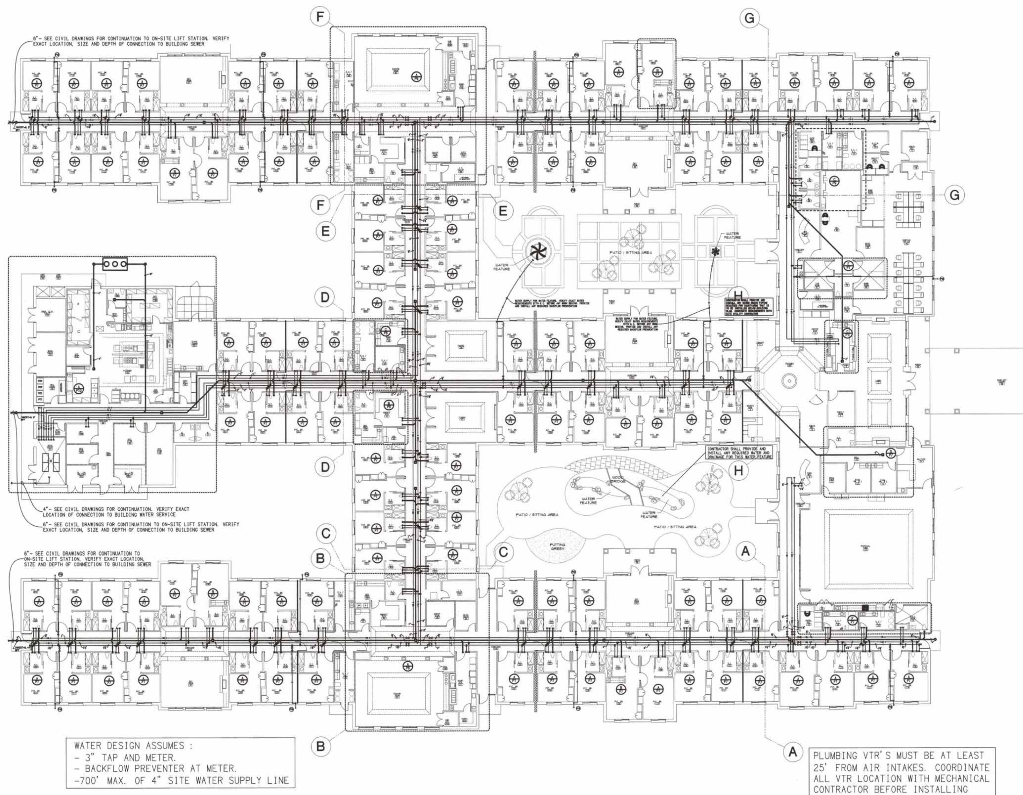
A P1 OVERALL PLUMBING PLAN SCALE: 1/16" = 1'-0"
