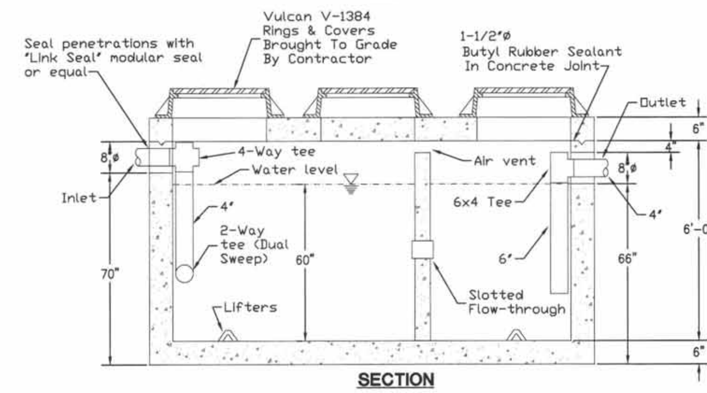
B P11 1500 GAL. GREASE INTERCEPTOR NO SCALE BY PLUMBING CONTRACTOR
