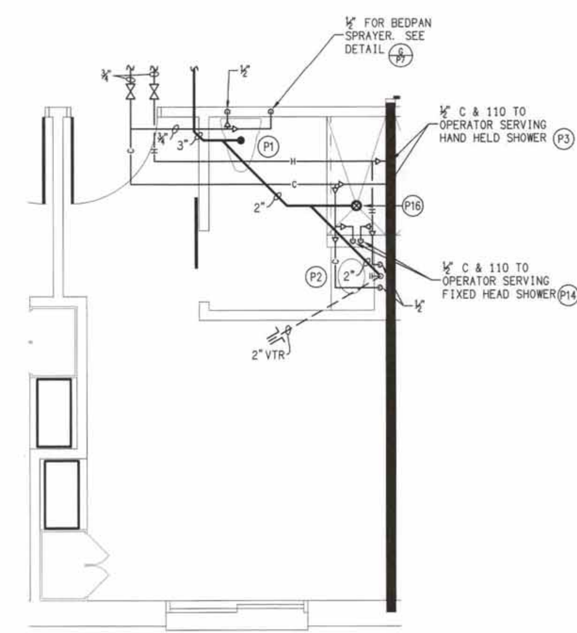
A ENLARGED PLUMBING PLAN P7 SCALE: 1/4" = 1'-0" TYPICAL ROOM
