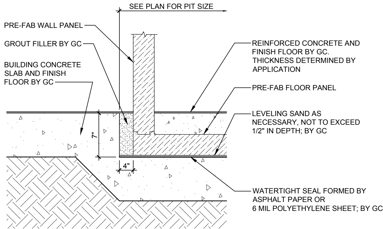
NOTE: RECESSED WALK-IN WALL AND FLOOR PANEL DETAIL APPLIES TO BOTH WALK-IN COOLER AND WALK-IN FREEZER 4 SCALE: NTS
