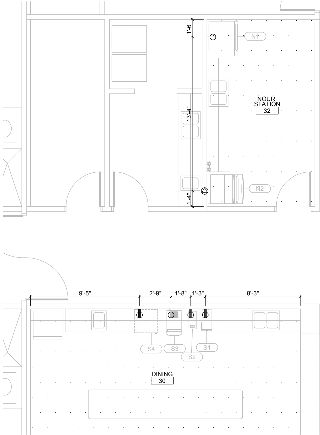
PLAN TRUE 2 NOURISH & DINING KITCHEN ELECTRICAL PLAN SCALE: 1/4" = 1'-0"
