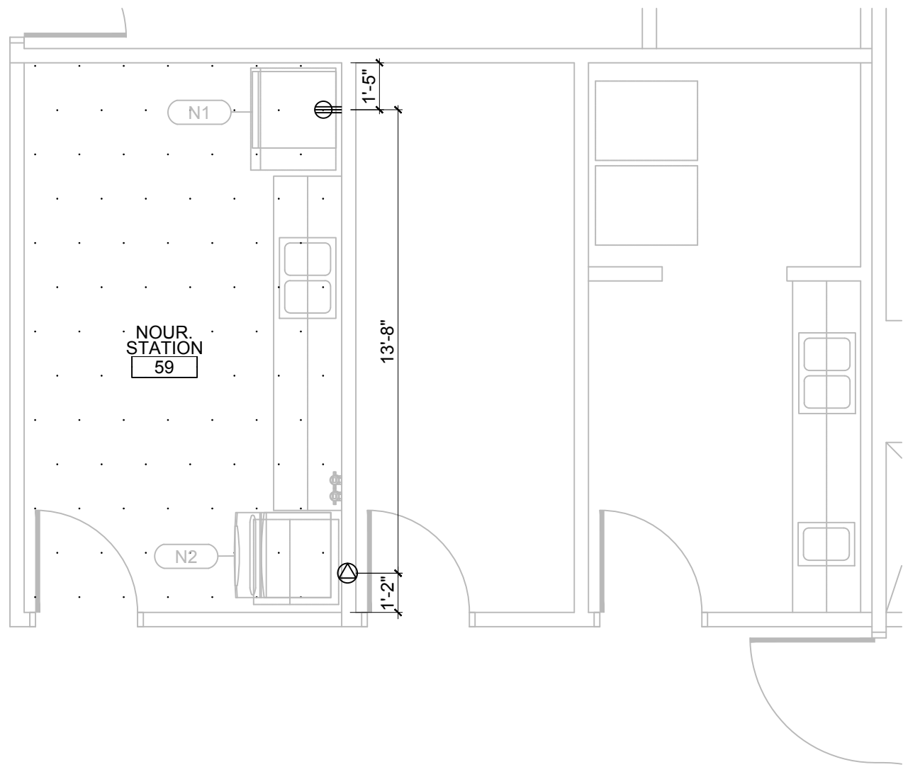
PLAN TRUE 2 NOURISH & DINING KITCHEN ELECTRICAL PLAN SCALE: 1/4" = 1'-0"
