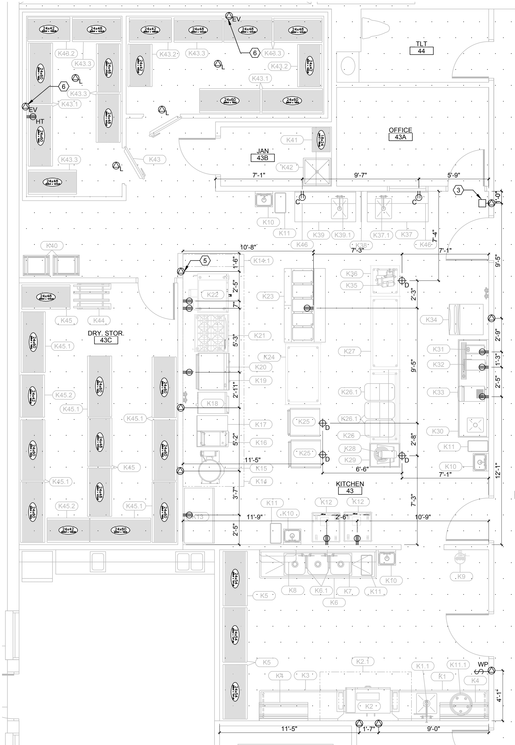
PLAN TRUE 1 MAIN KITCHEN ELECTRICAL PLAN SCALE: 1/4" = 1'-0"
