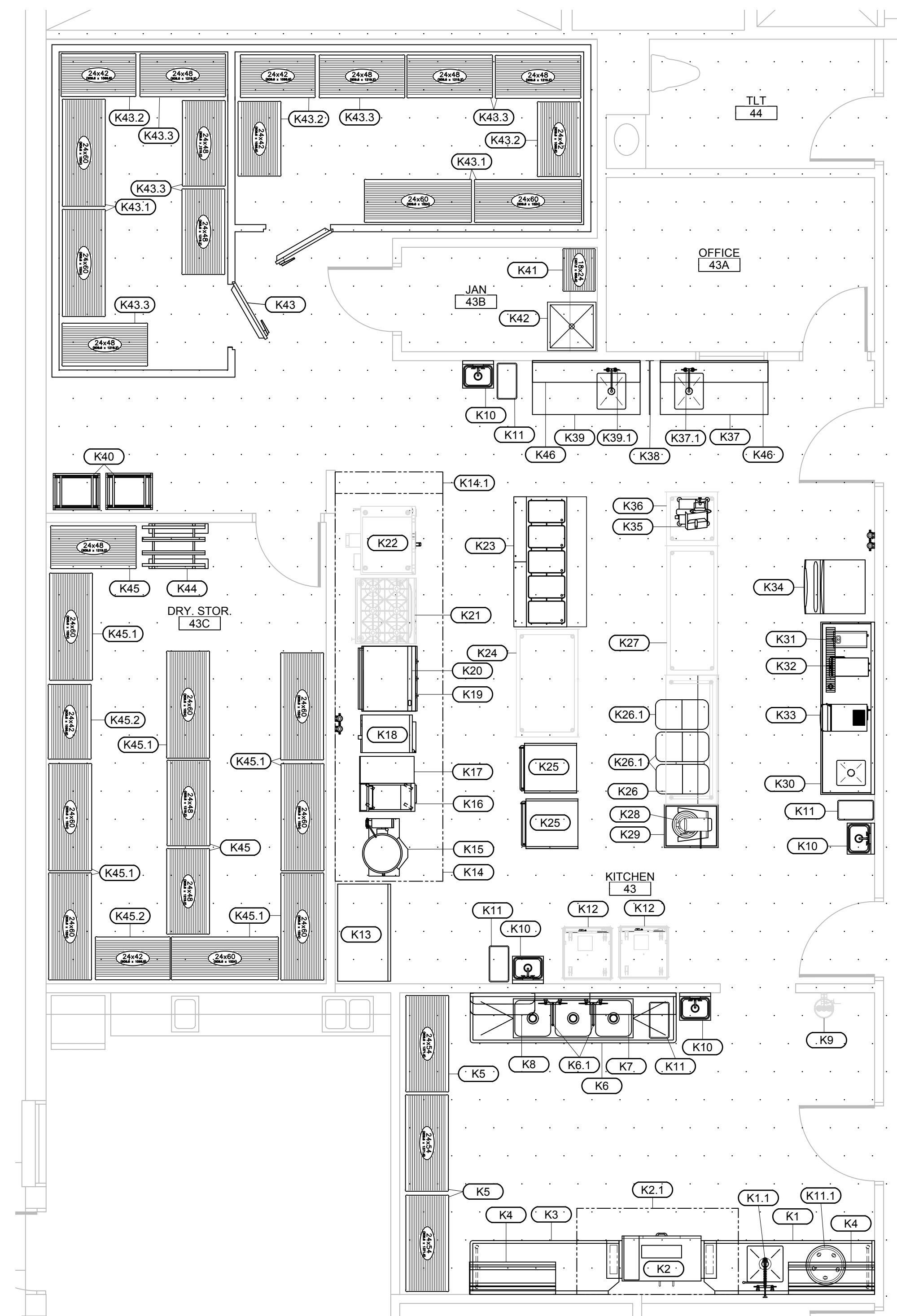
PLAN TRUE 1 MAIN KITCHEN EQUIPMENT PLAN SCALE: 1/4" = 1'-0"
