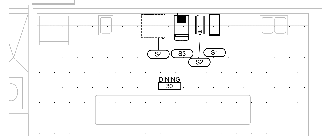
PLAN TRUE 2 NOURISH & DINING KITCHEN EQUIPMENT PLAN SCALE: 1/4" = 1'-0"
