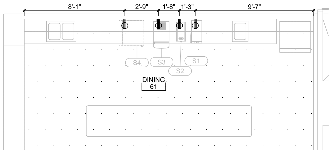
PLAN TRUE 3 NOURISH & DINING KITCHEN ELECTRICAL PLAN SCALE: 1/4" = 1'-0"
