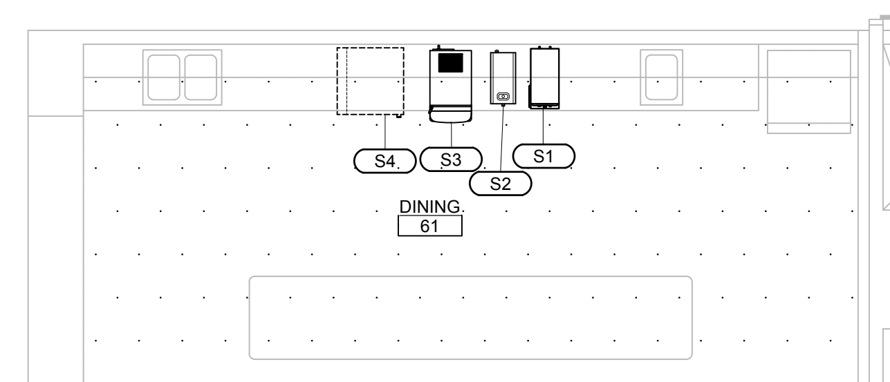
PLAN TRUE 3 NOURISH & DINING KITCHEN EQUIPMENT PLAN SCALE: 1/4" = 1'-0"
