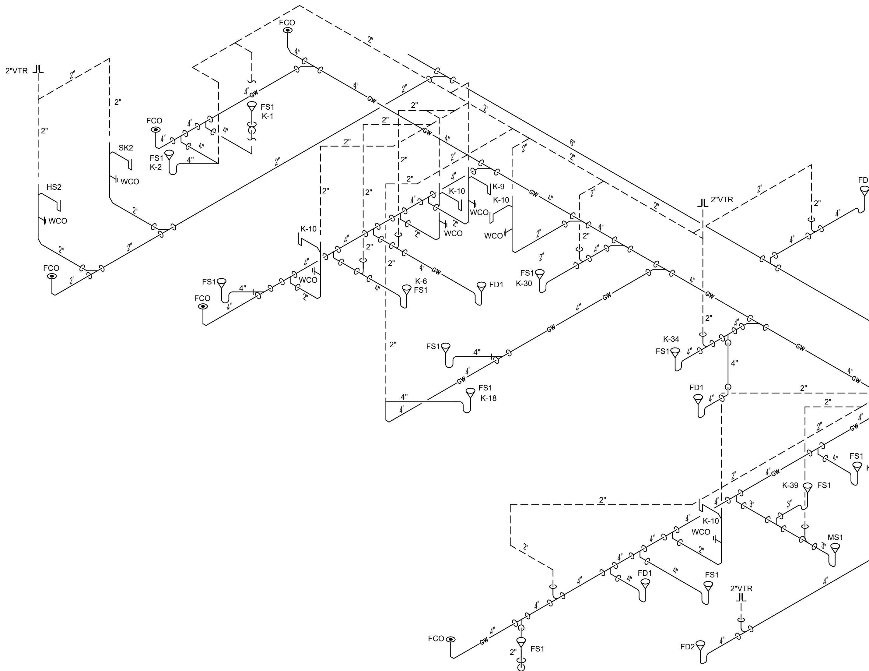
6- KITCHEN WASTE-VENT RISER DIAGRAM No Scale
