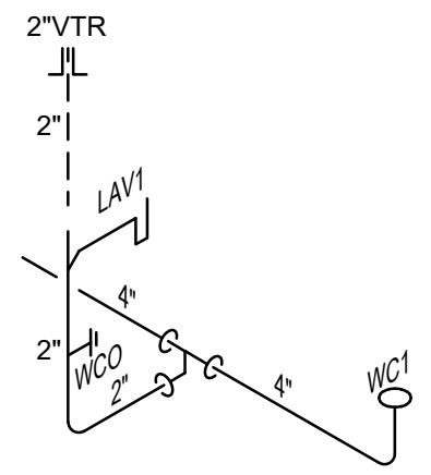
8 - WASTE-VENT RISER DIAGRAM TYPICAL STAFF LOUNGE NO SCALE
