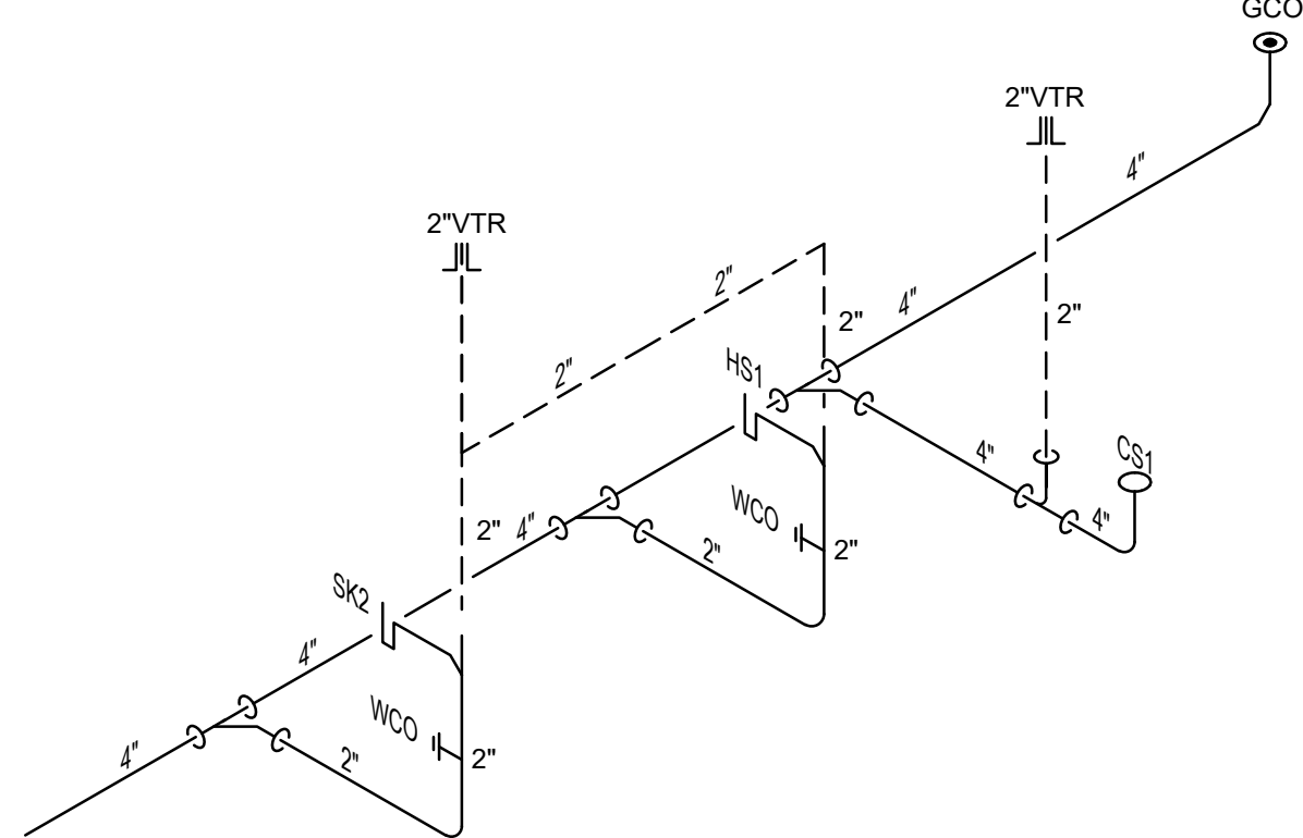
4 - WASTE-VENT RISER DIAGRAM TYPICAL PRIVATE S.U./S.L. ROOM NO SCALE
