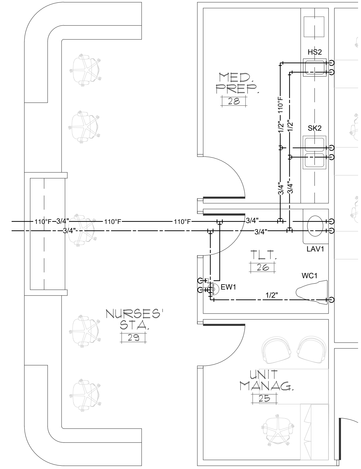
3 PARTIAL DOMESTIC WATER PLAN 1/4" = 1'-0"
