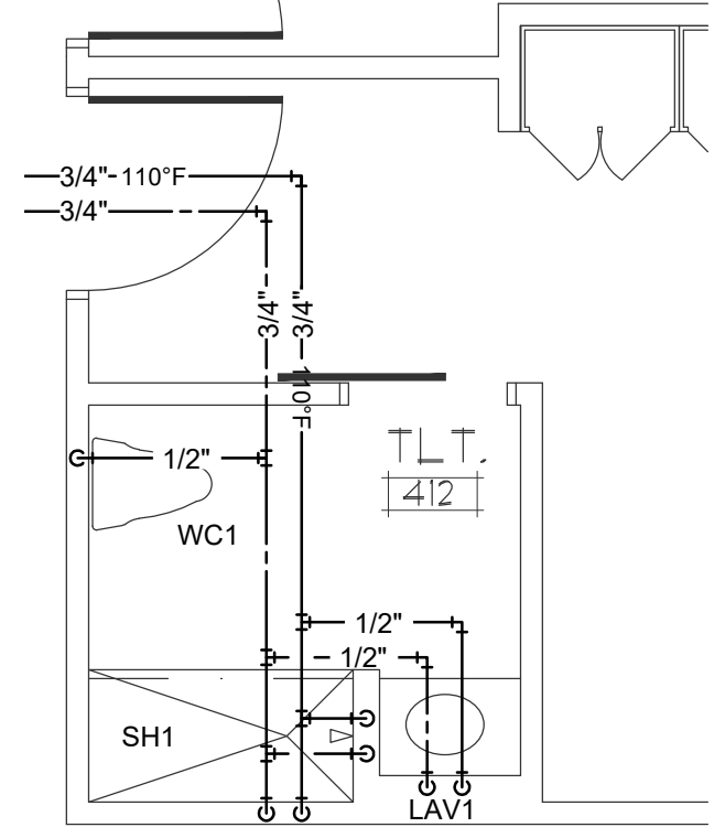
5 PARTIAL DOMESTIC WATER PLAN 1/4" = 1'-0"
