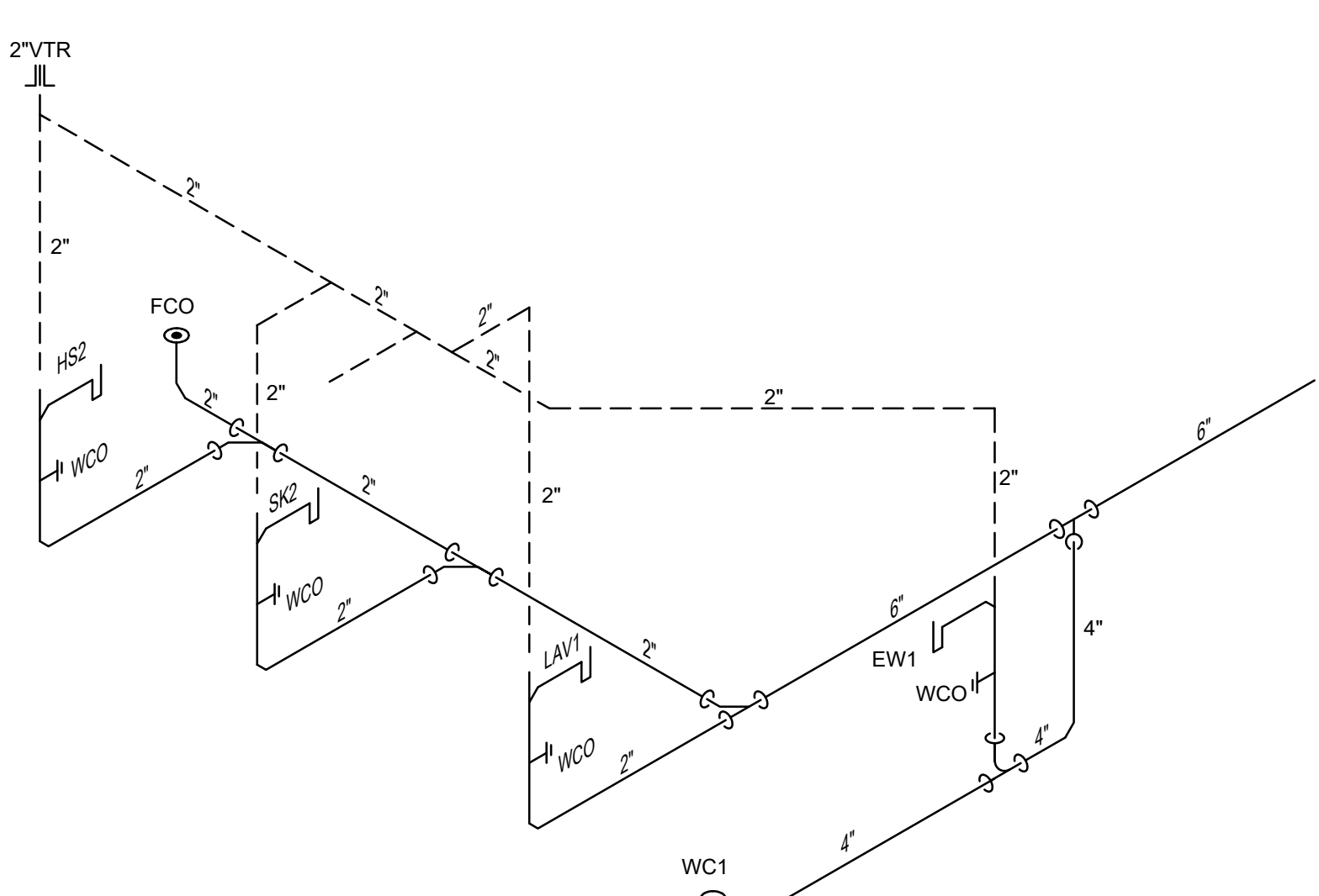
3 - WASTE-VENT RISER DIAGRAM TYPICAL NURSES STATION NO SCALE
