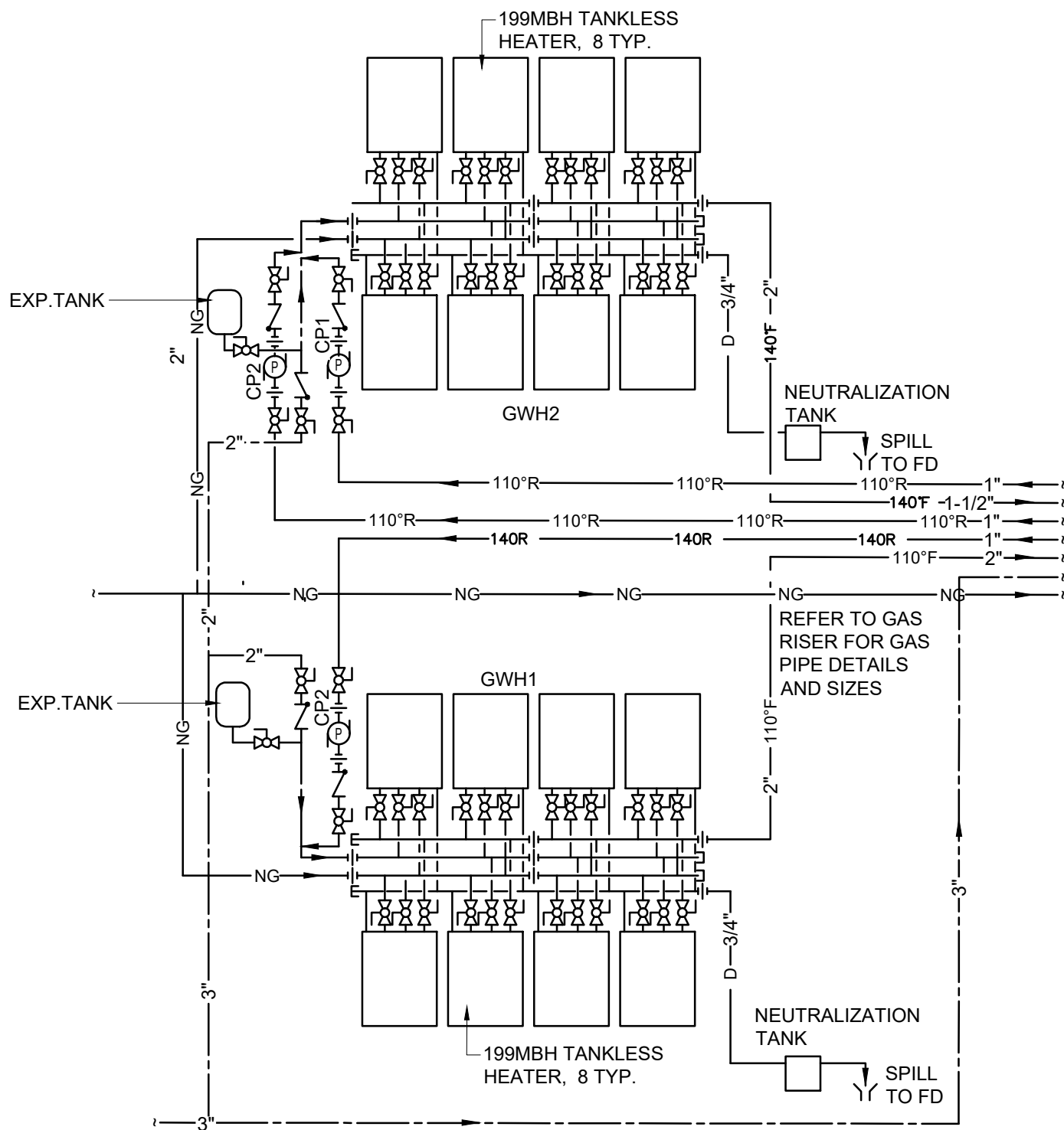
5 - DOMESTIC WATER HEATER PIPING DETAIL NOT TO SCALE
