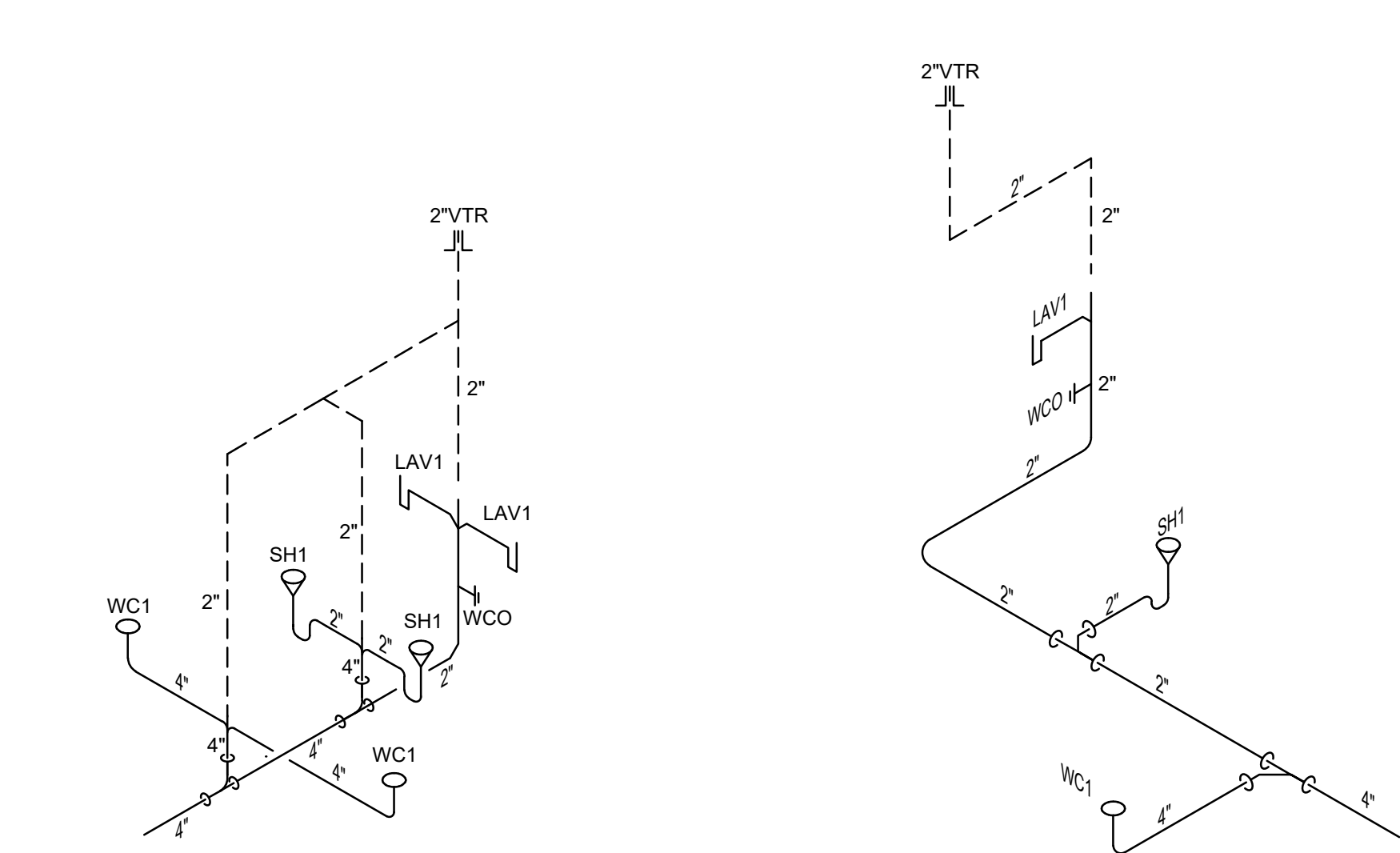
1 - WASTE-VENT RISER DIAGRAM TYPICAL PRIVATE BEDROOM (SUITE) NO SCALE
