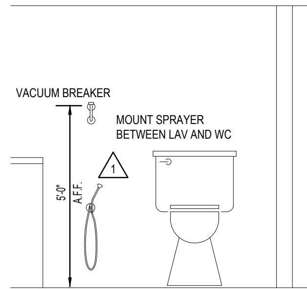
13 - BEDPAN CLEANSER DETAIL NOT TO SCALE
