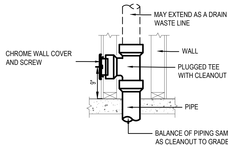
WALL CLEANOUT (WCO)
