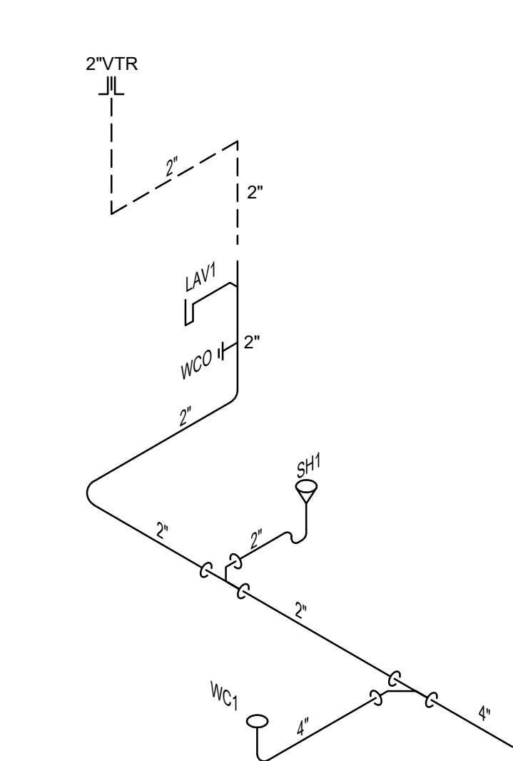
2 - WASTE-VENT RISER DIAGRAM TYPICAL PRIVATE BEDROOM NO SCALE
