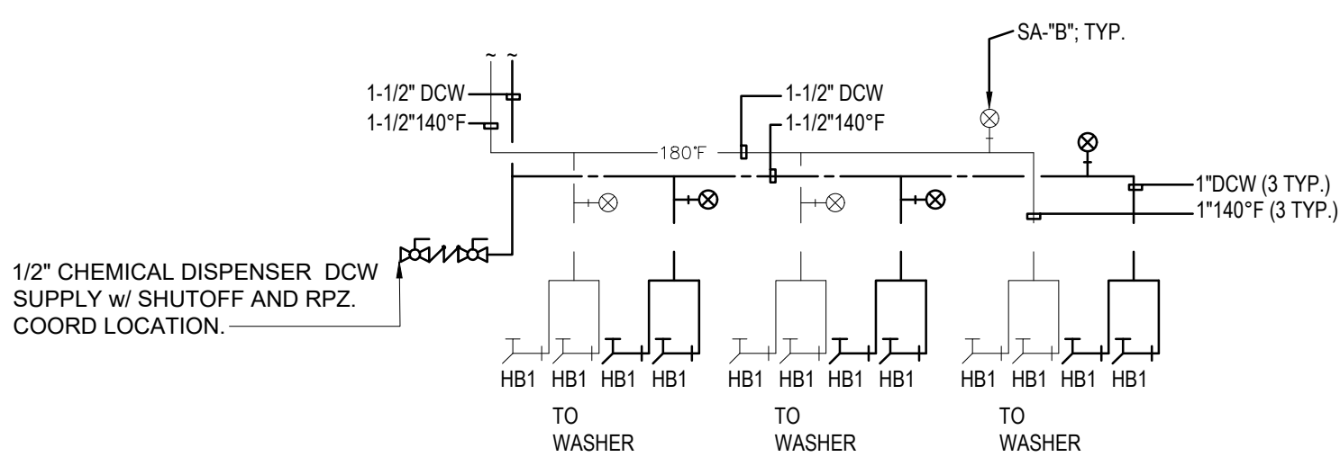
2 - COMMERCIAL WASHER WATER CONNECTION DETAIL NOT TO SCALE
