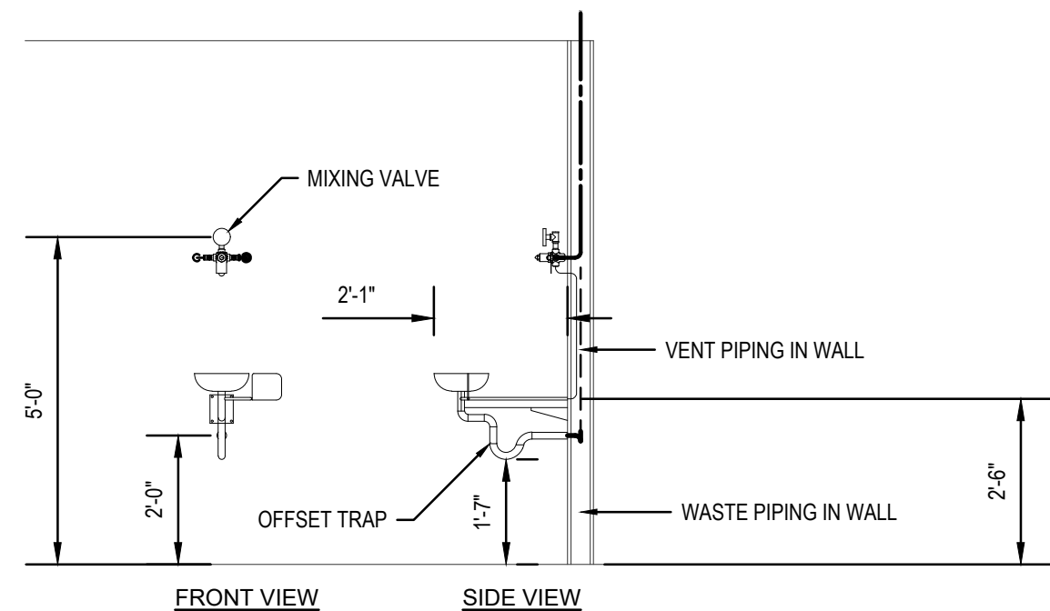
11 - WALL MOUNTED EYEWASH DETAIL NOT TO SCALE
