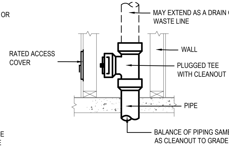
WALL CLEANOUT (WCO) RATED WALL
