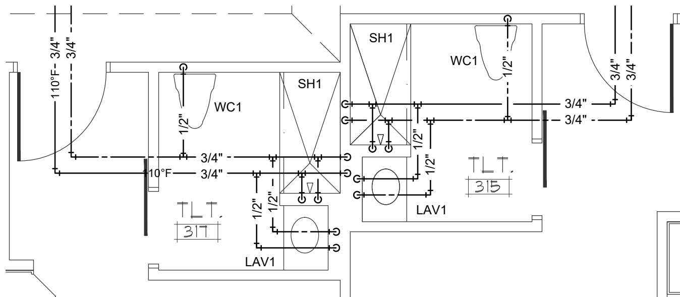
6 PARTIAL DOMESTIC WATER PLAN 1/4" = 1'-0"
