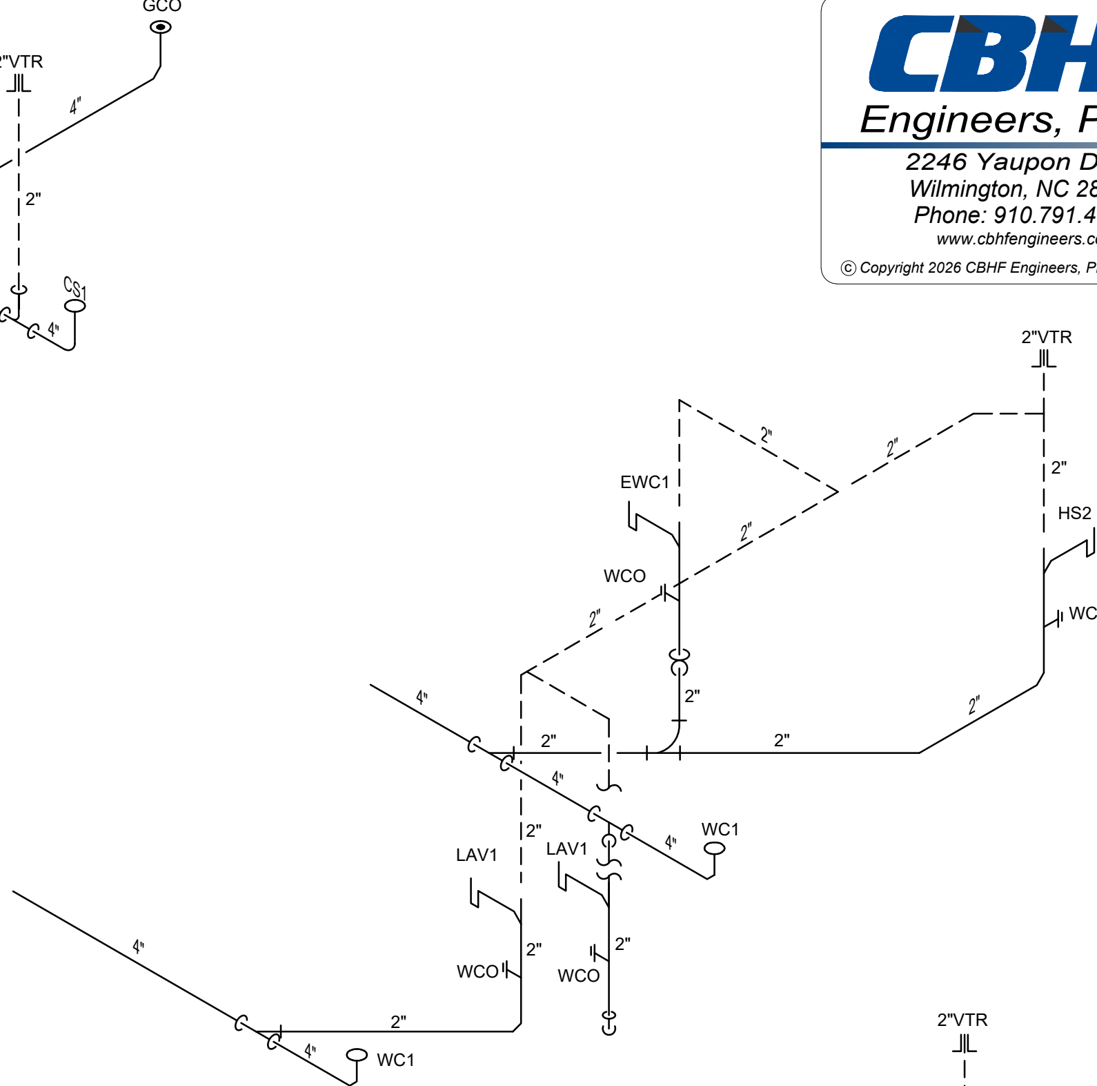
5 - WASTE-VENT RISER DIAGRAM TYPICAL PUBLIC RESTROOM AND WORK RM NO SCALE
