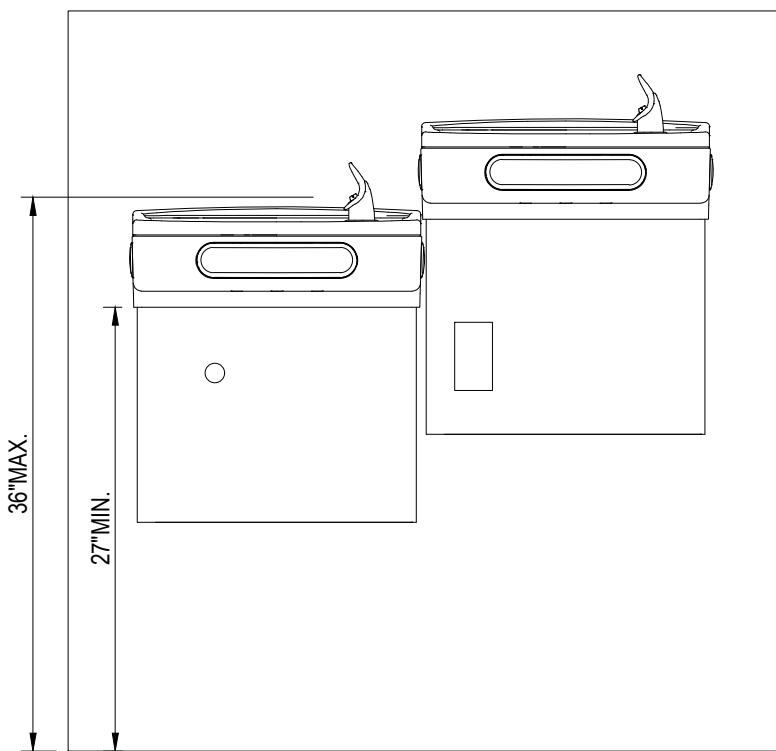
9 - TYPICAL BI-LEVEL WATER COOLER DETAIL NOT TO SCALE
