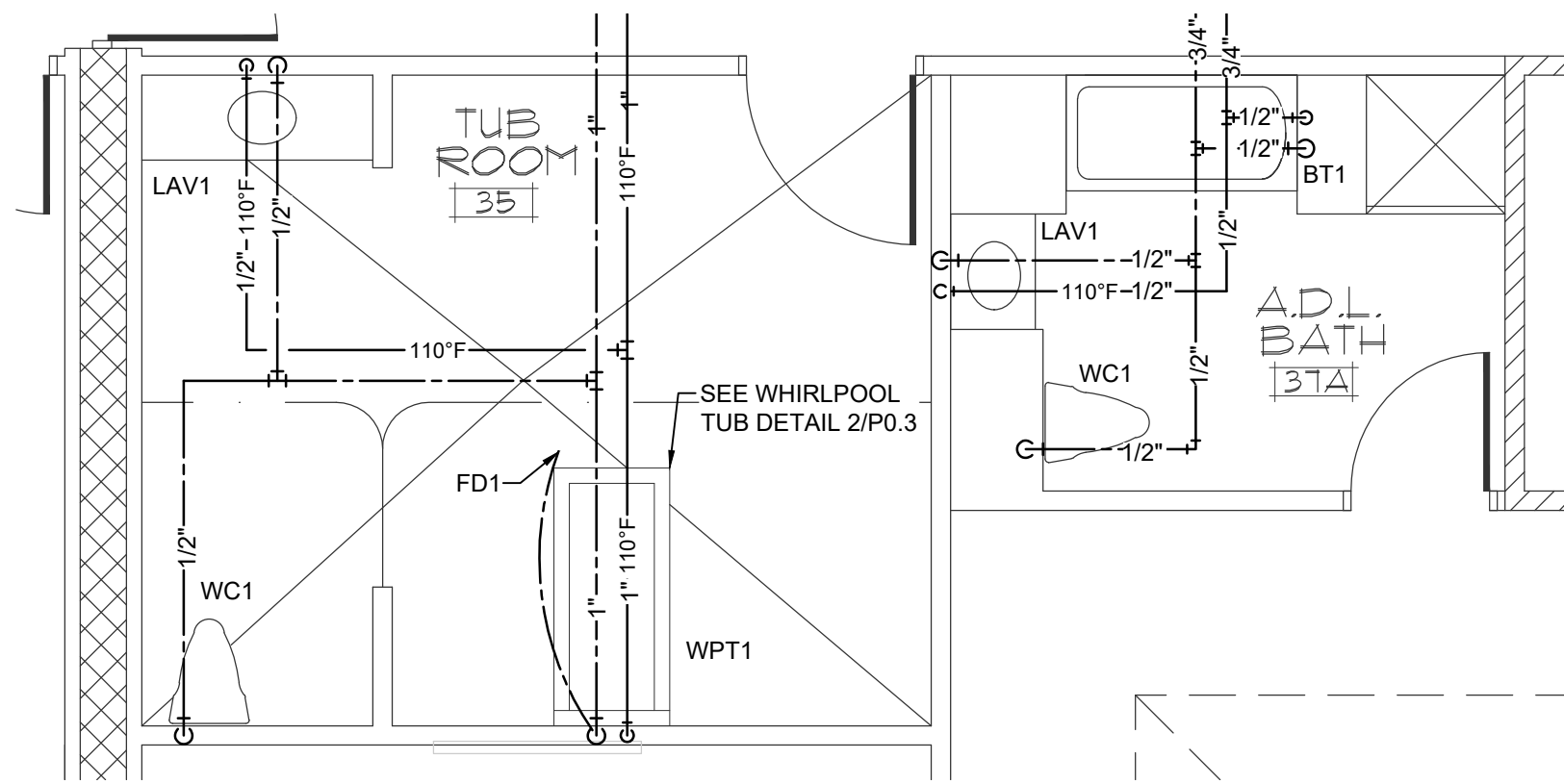
2 PARTIAL DOMESTIC WATER PLAN 1/4" = 1'-0"
