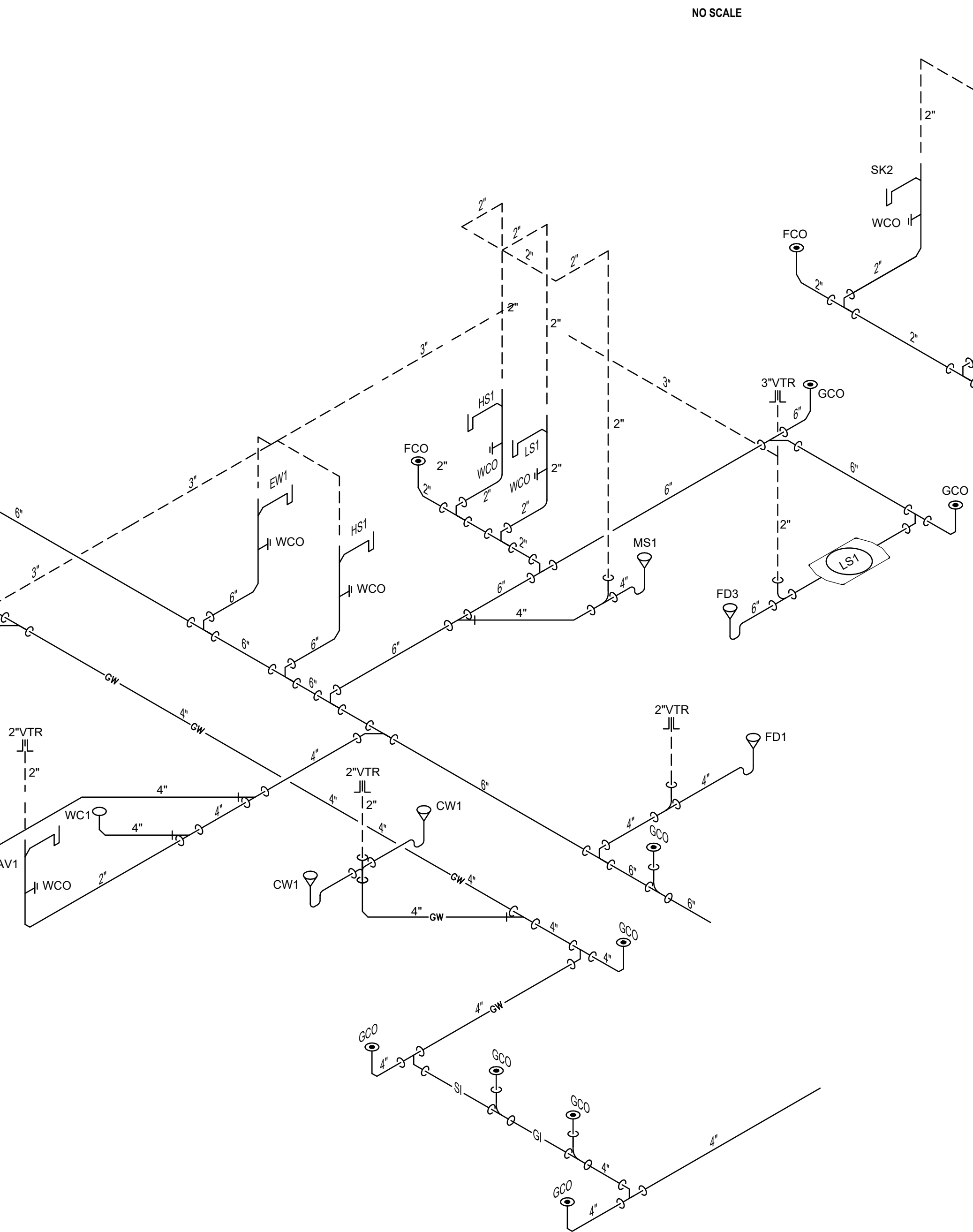
5 - WASTE-VENT RISER DIAGRAM TYPICAL PUBLIC RESTROOM AND WORK RM NO SCALE
