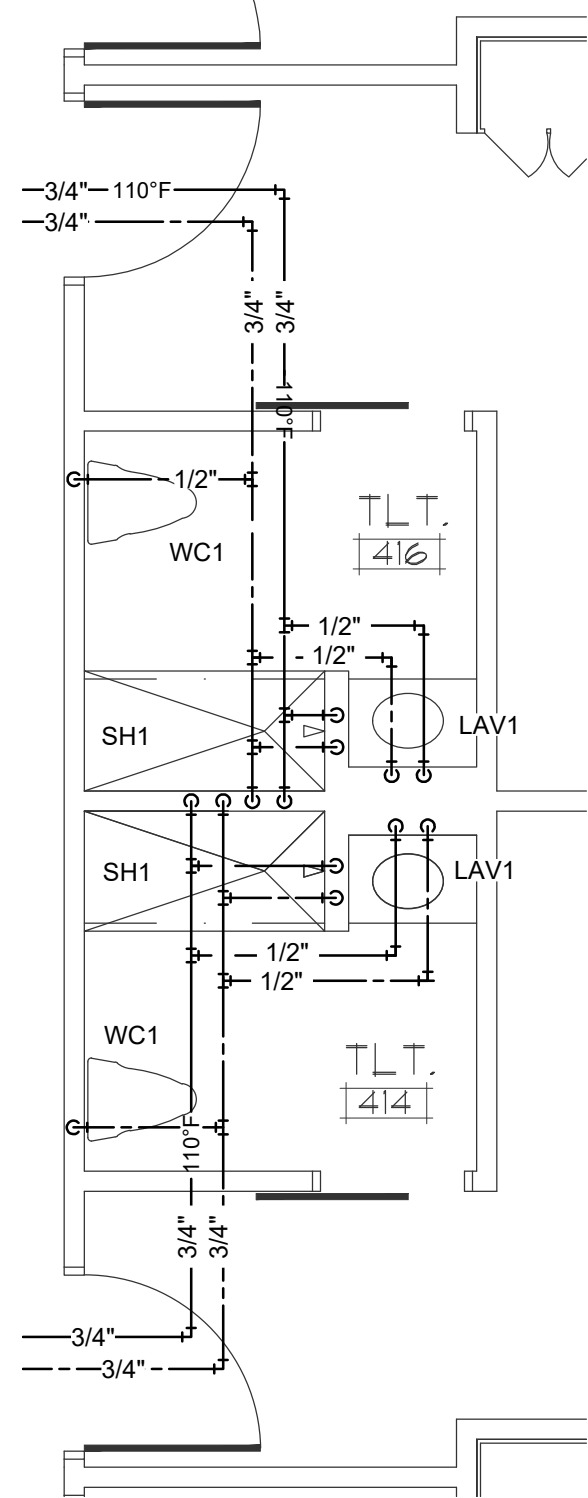
4 PARTIAL DOMESTIC WATER PLAN 1/4" = 1'-0"
