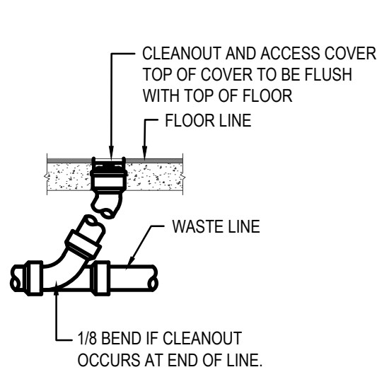
FLOOR CLEANOUT (FCO)
