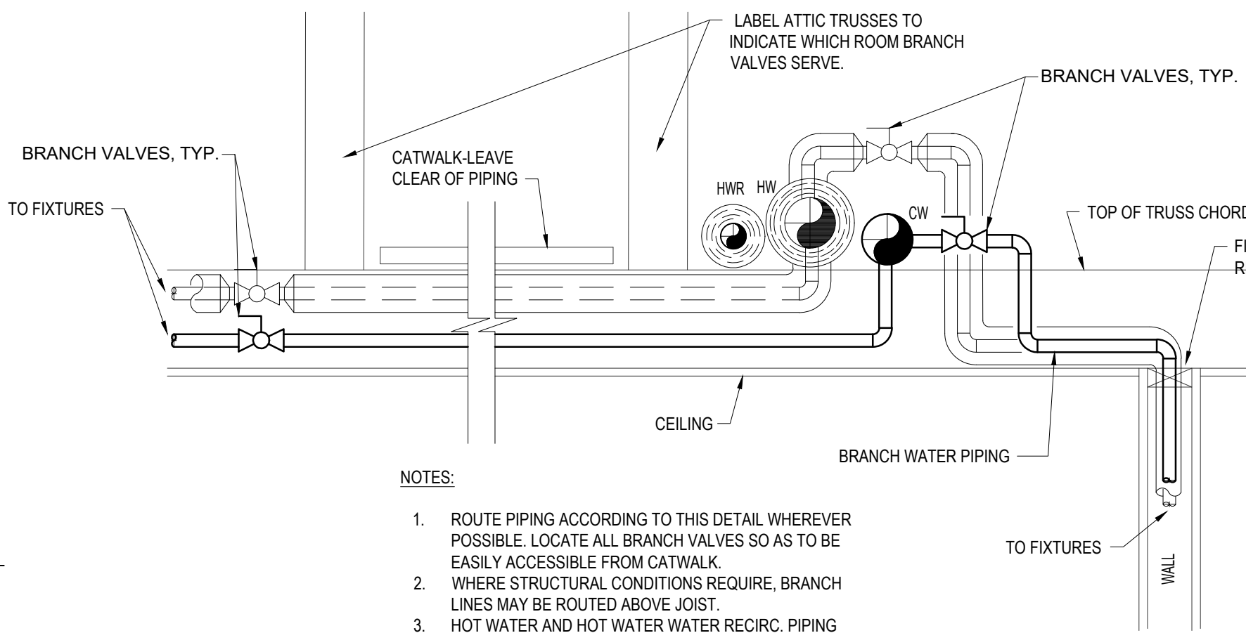
8 - ATTIC WATER PIPING DETAIL NOT TO SCALE
