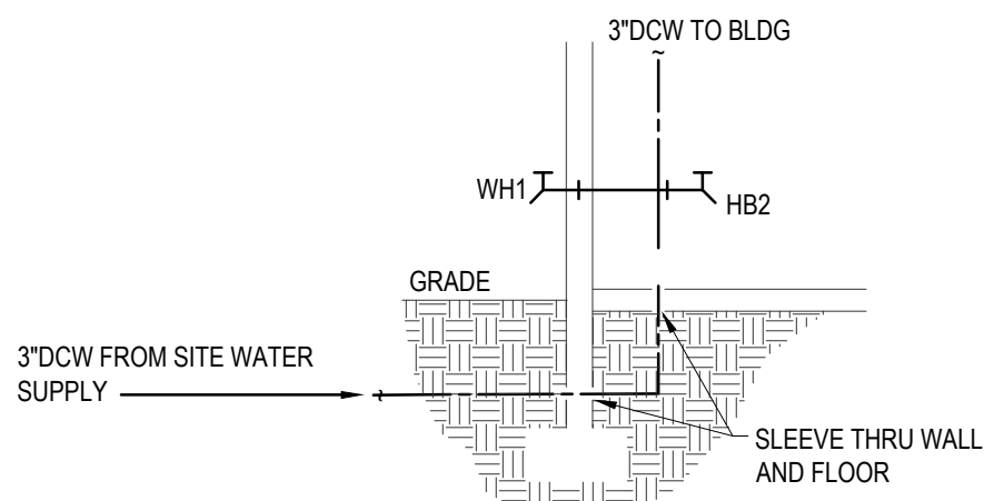
7 - WATER SERVICE ENTRANCE DETAIL NOT TO SCALE
