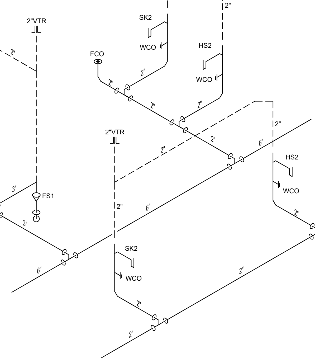
5 - WASTE-VENT RISER DIAGRAM TYPICAL PUBLIC RESTROOM AND WORK RM NO SCALE
