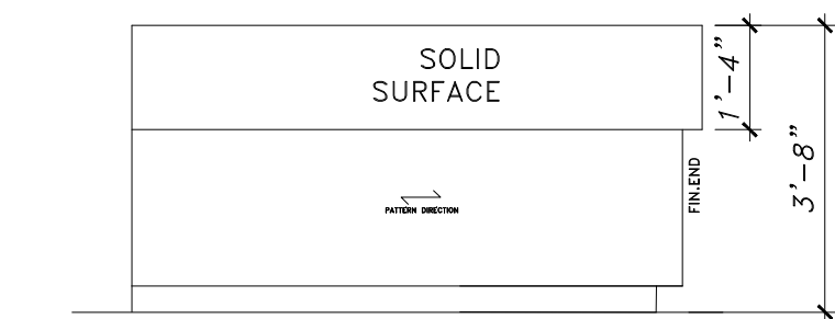
2 NURSE STATION (100, 106) - DESK SCALE: 3/8" = 1'-0"
