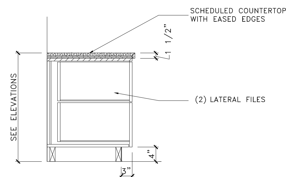
4 Rec Desk - Lateral Files SCALE: 3/4" = 1'-0"
