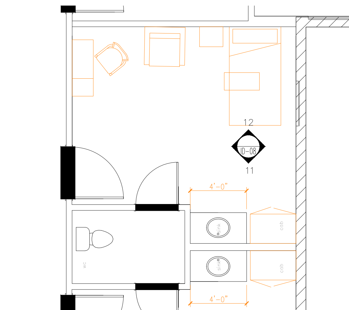
10 EAST HALL - PRIVATE ROOM TYP. SCALE: 3/8" = 1'-0"
