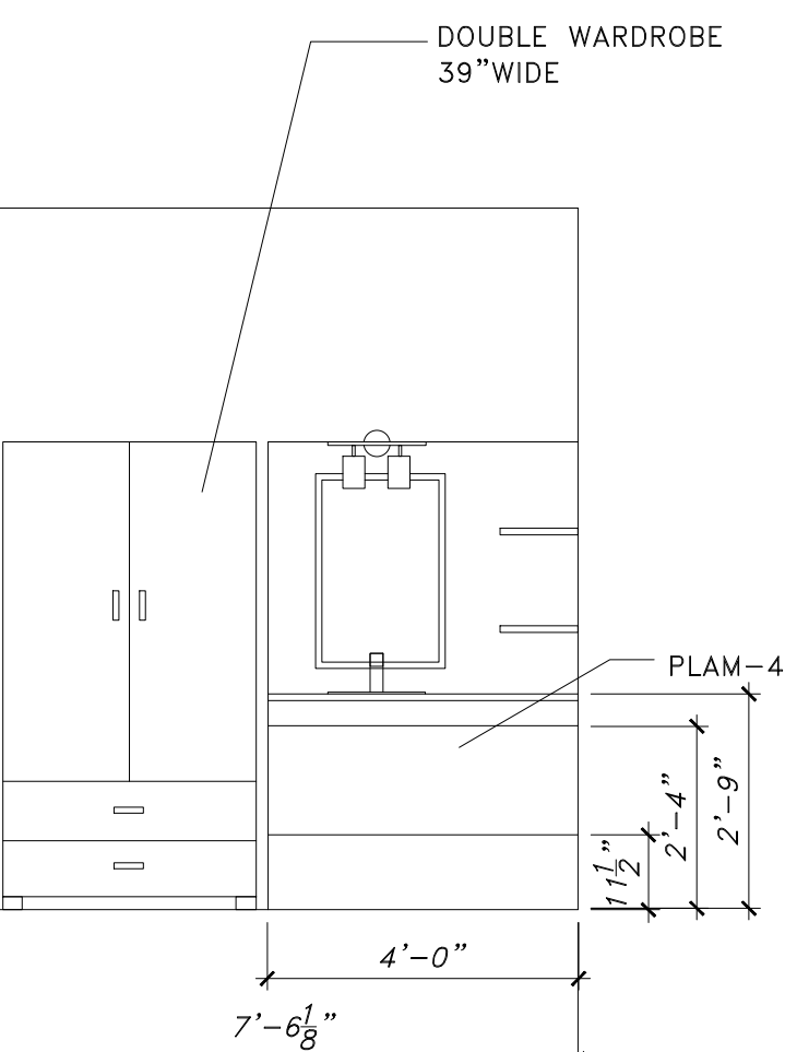
11 EAST HALL - PRIVATE ROOM TYP. SCALE: 3/8" = 1'-0"
