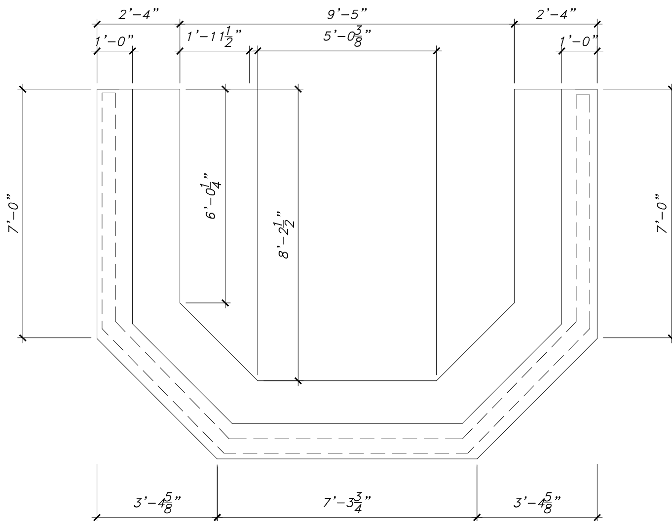
11 NURSE STATION (100, 106) - DESK PLAN SCALE: 3/8" = 1'-0"
