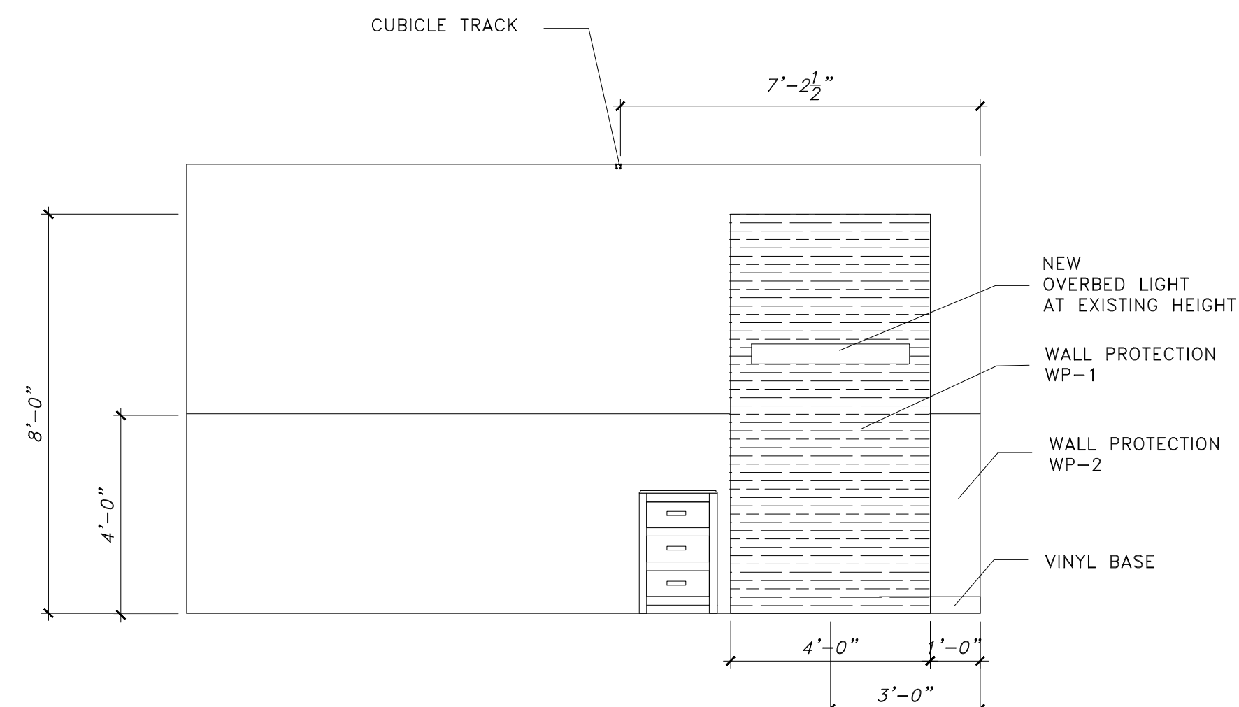
12 EAST HALL - PRIVATE ROOM TYP. SCALE: 3/8" = 1'-0"
