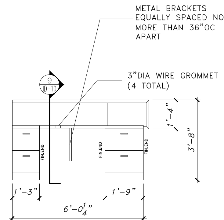
4 NURSE STATION (100, 106) - DESK SCALE: 3/8" = 1'-0"
