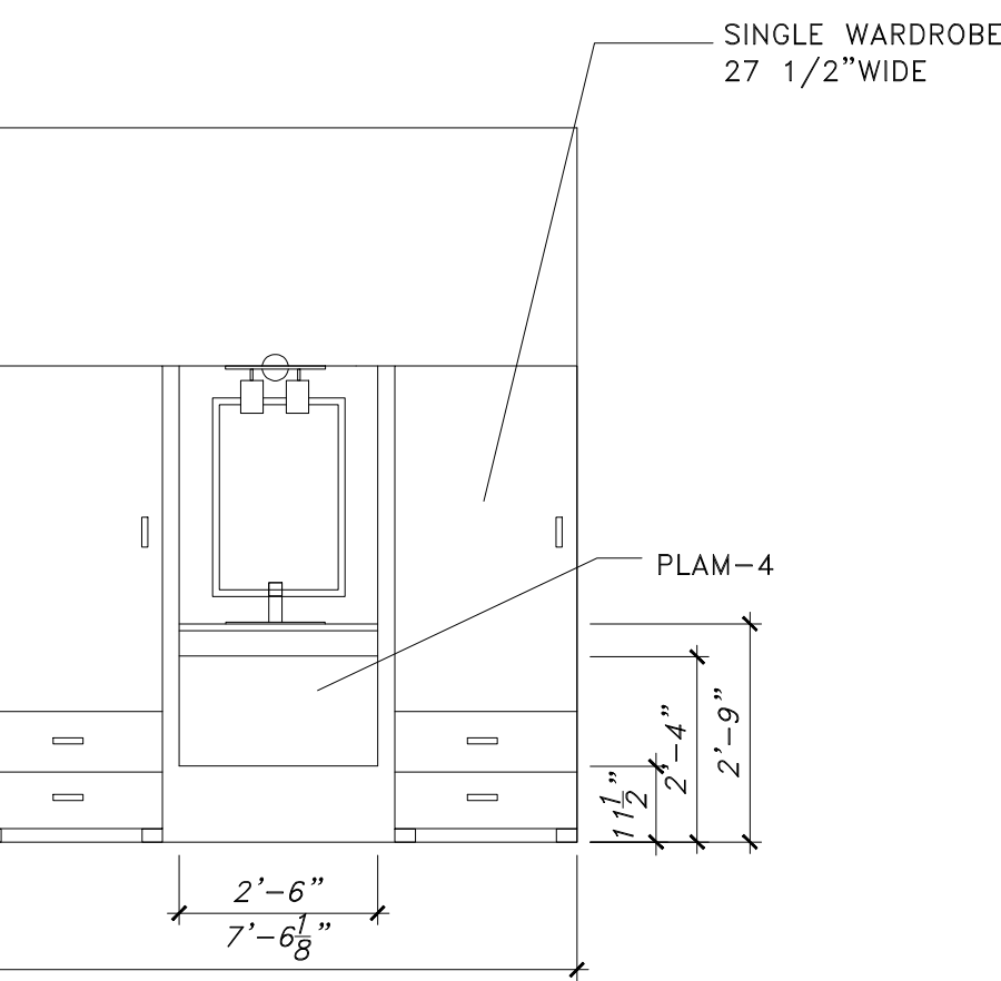
7 EAST HALL - SEMI-PRIVATE ROOM TYP. SCALE: 3/8" = 1'-0"
