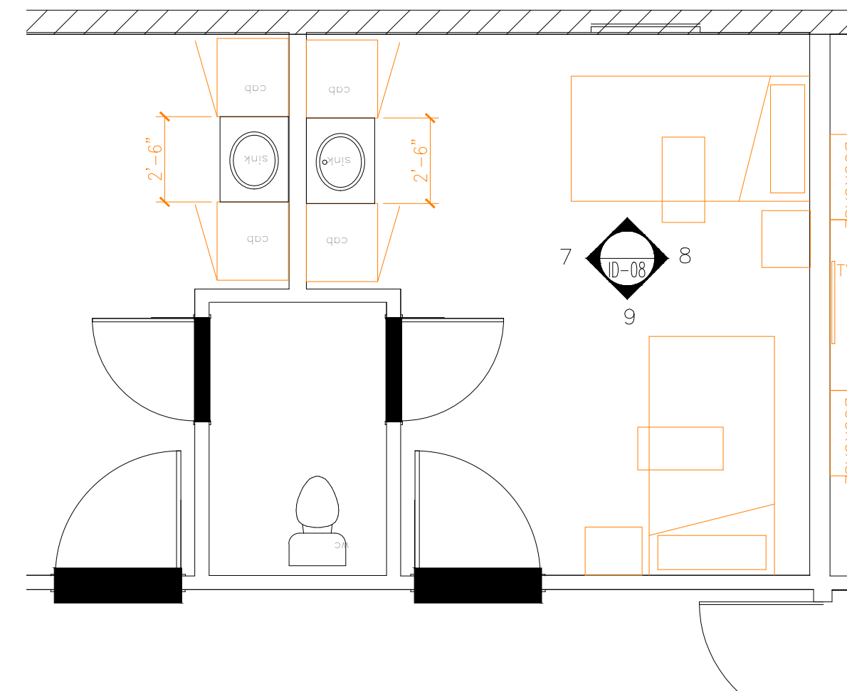
6 EAST HALL - SEMI-PRIVATE ROOM TYP. SCALE: 1/4" = 1'-0"
