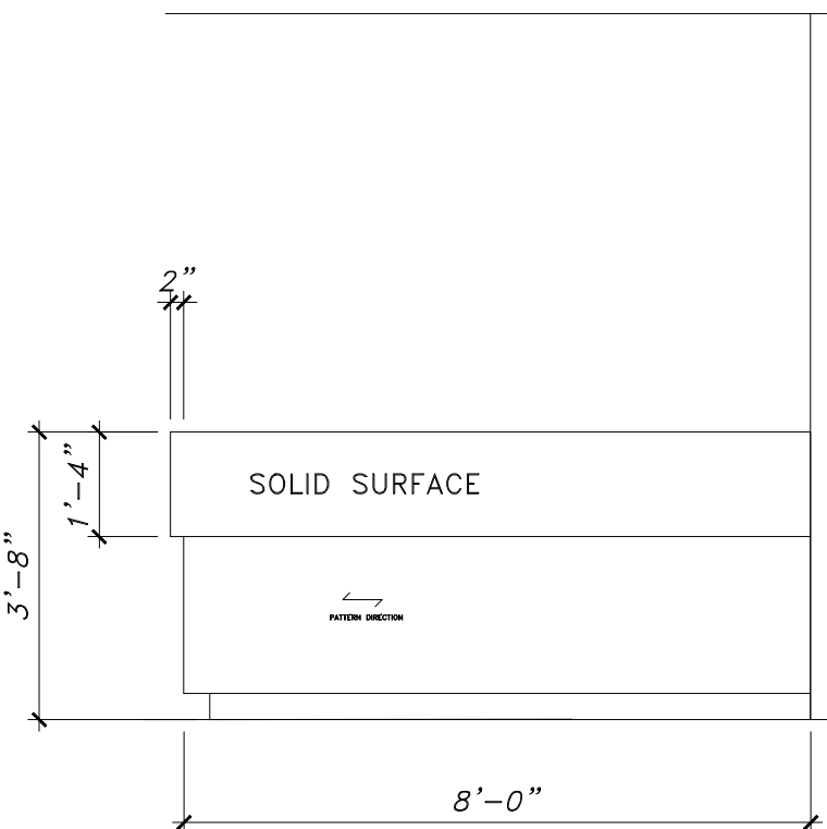
3 NURSE STATION (54) - DESK SCALE: 3/8" = 1'-0"
