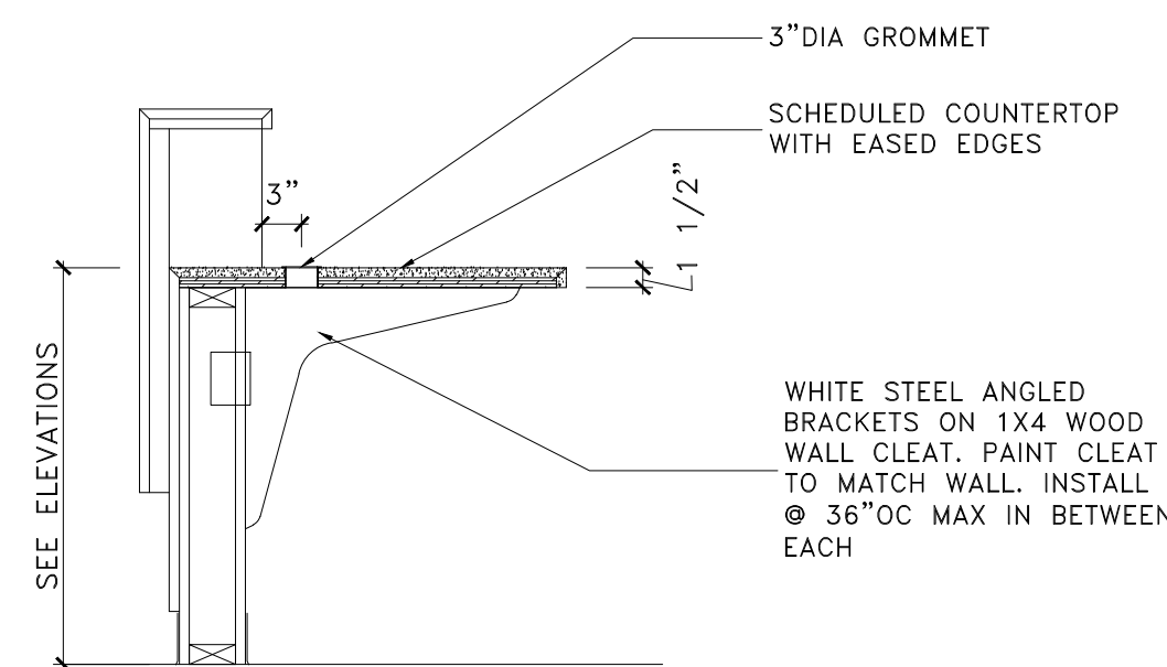
6 Rec Desk - Transaction Top SCALE: 3/4" = 1'-0"
