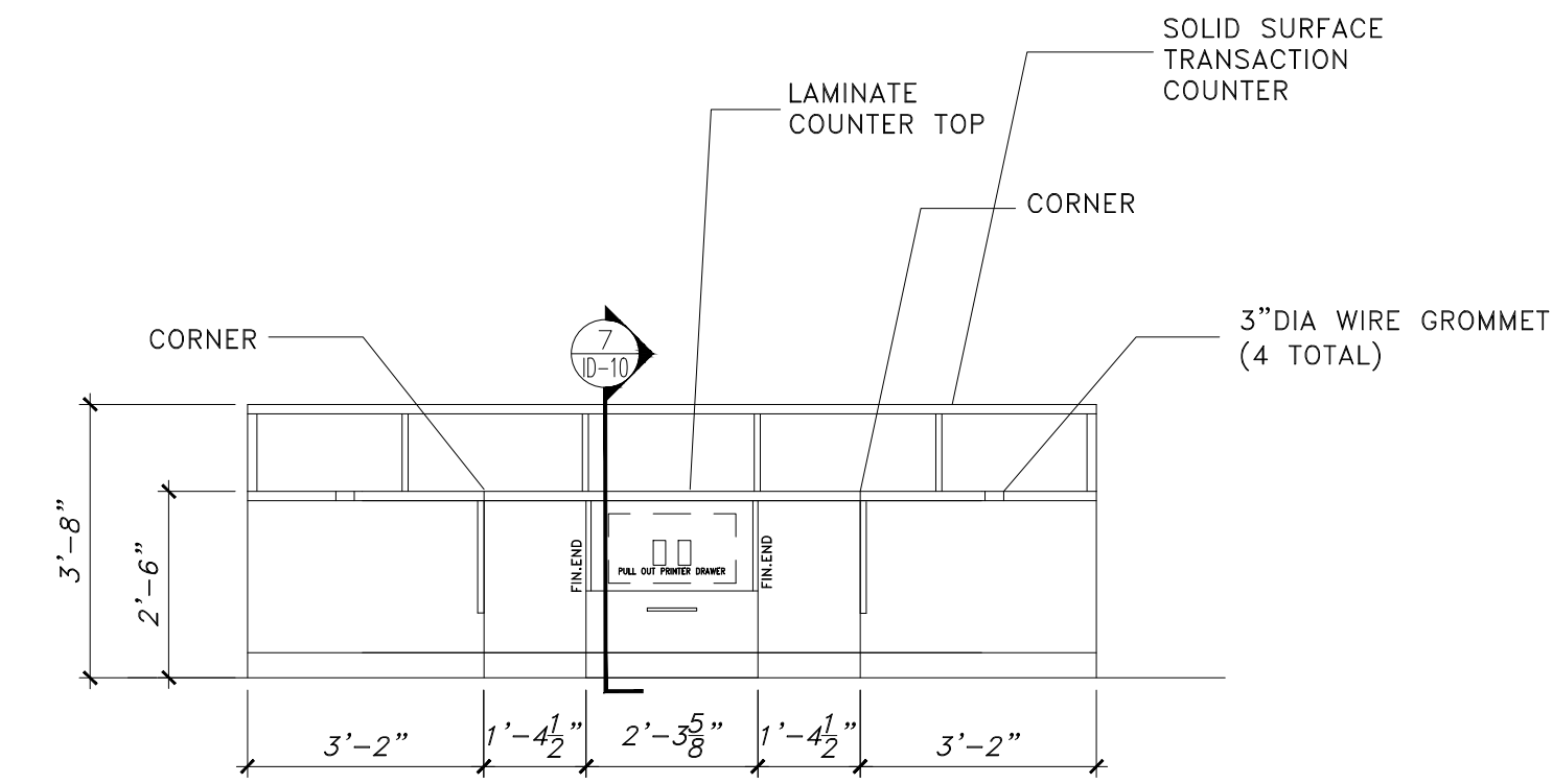
3 NURSE STATION (100, 106) - DESK SCALE: 3/8" = 1'-0"
