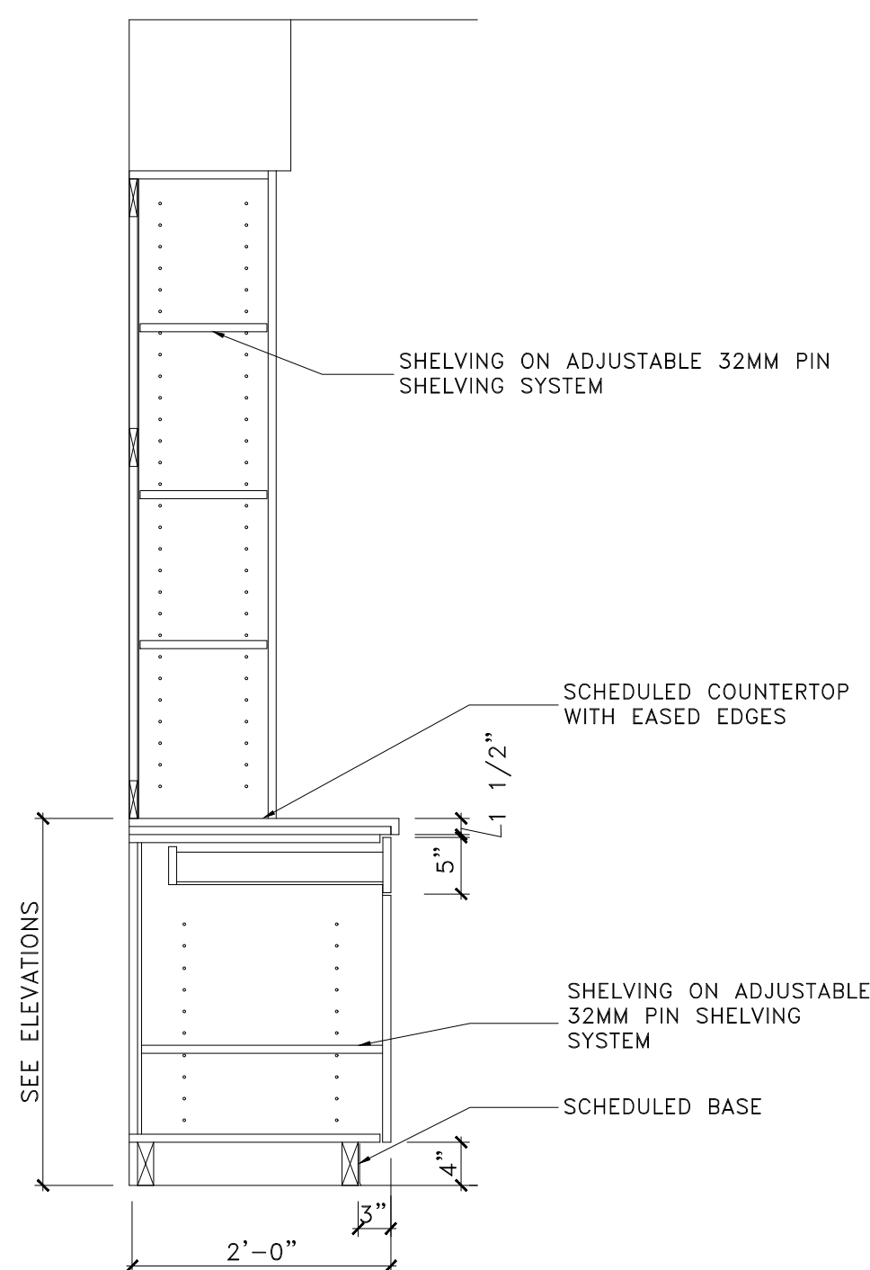
Speech Therapy - Bookcase
