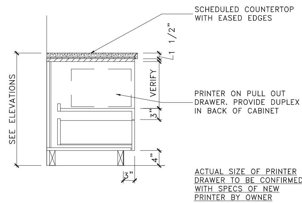
3 Rec Desk - Printer Drawer SCALE: 3/4" = 1'-0"
