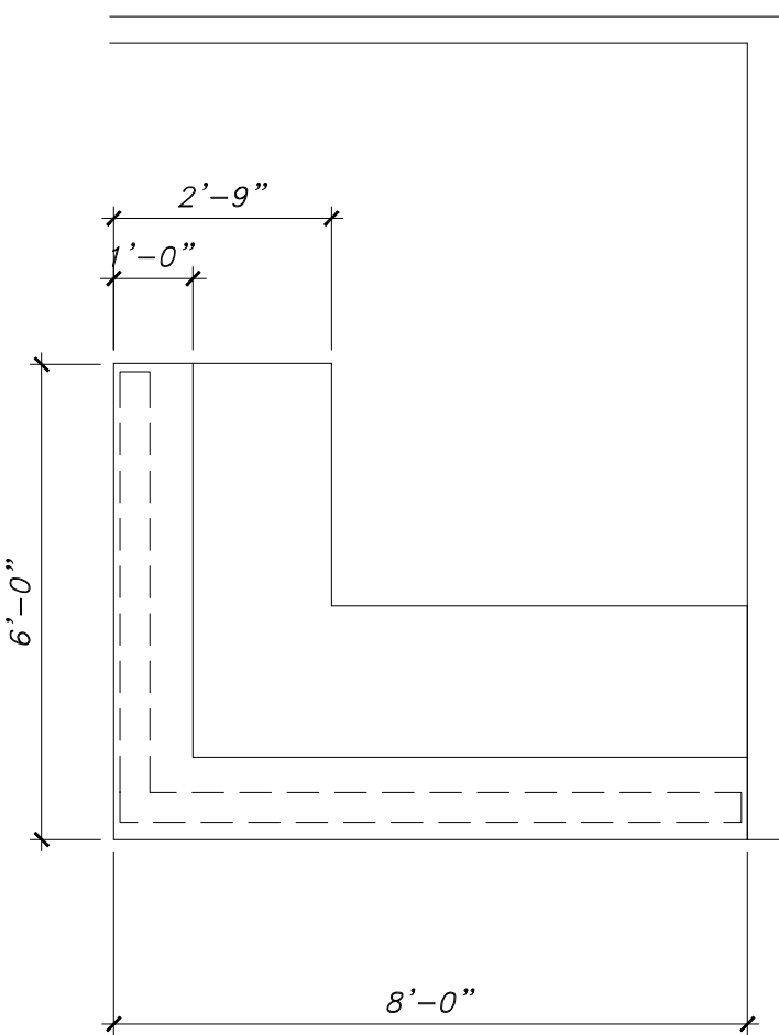
2 NURSE STATION (54) - DESK PLAN SCALE: 3/8" = 1'-0"
