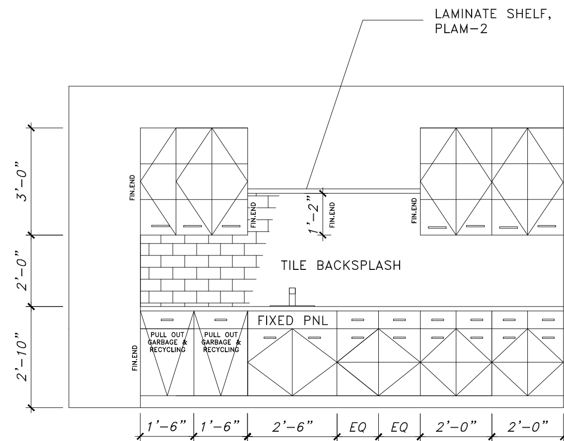
10 ACTIVITY ROOM (104) - CABINETRY SCALE: 3/8" = 1'-0"
