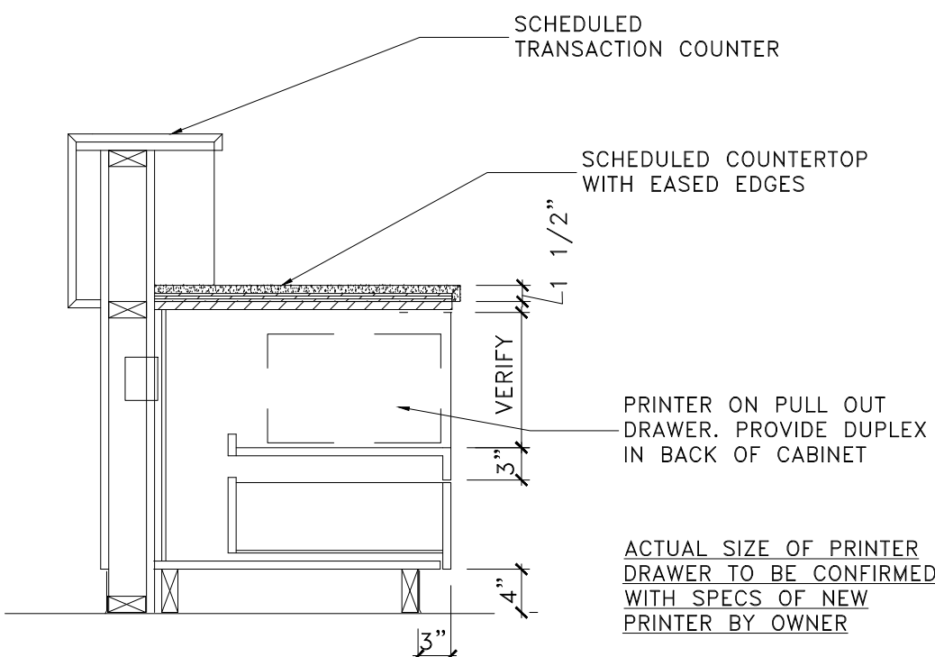
Nurse Desk - Printer Drawer SCALE: \frac{3}{4}" = 1'-0"
