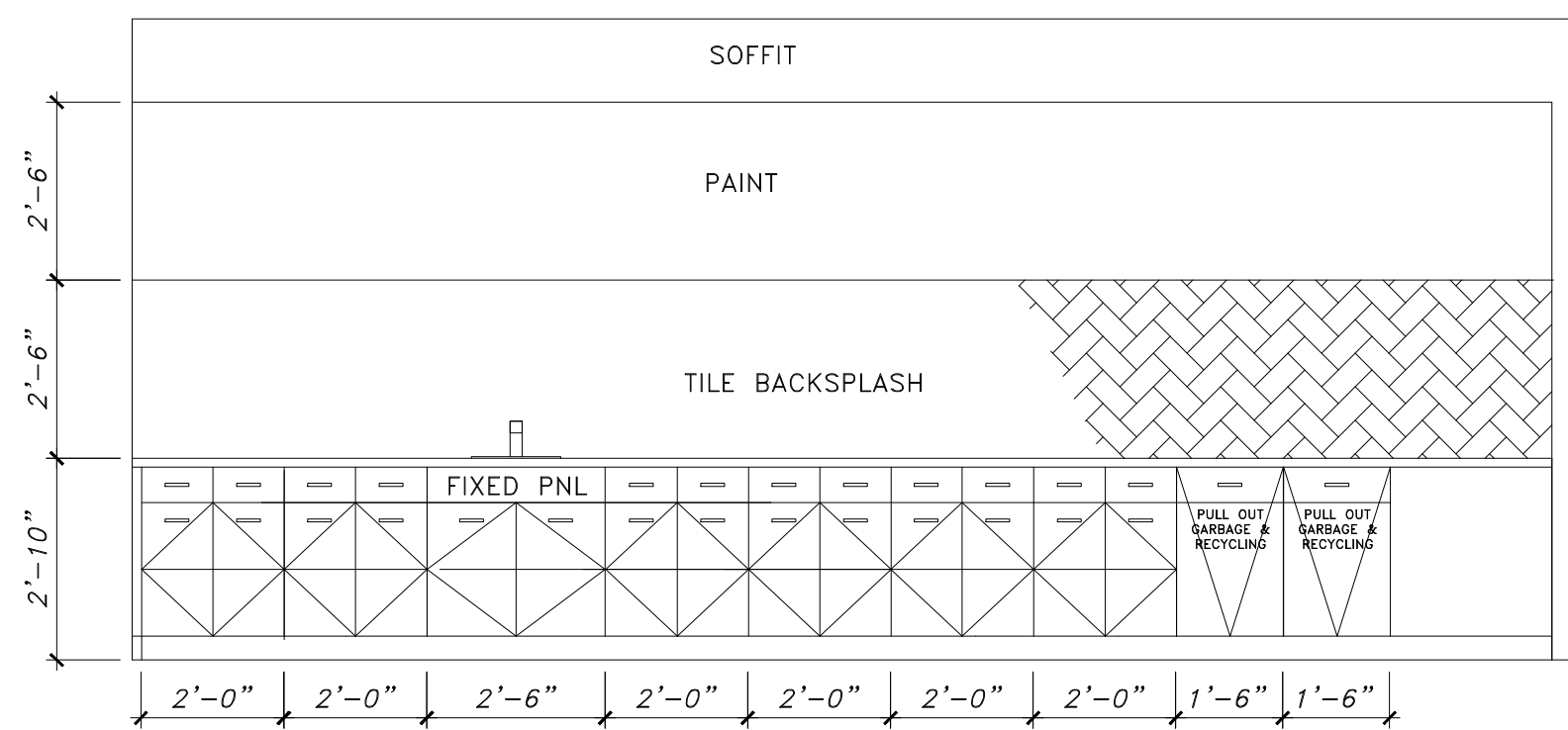
7 DINING ROOM (84) - CABINETRY SCALE: 3/8" = 1'-0"
