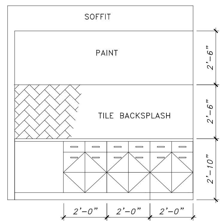
DINING ROOM (84) - CABINETRY SCALE: 3/8" = 1'-0"
