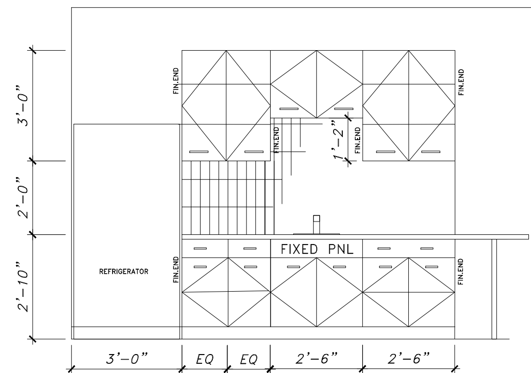
9 EMPLOYEE LOUNGE (92) - CABINETRY SCALE: 3/8" = 1'-0"
