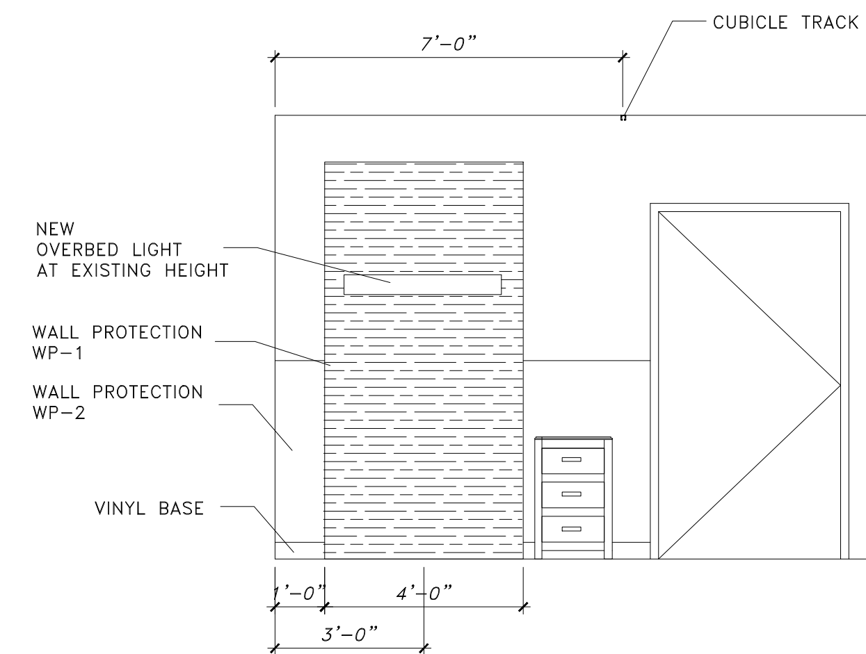
9 EAST HALL - SEMI-PRIVATE ROOM TYP. SCALE: 3/8" = 1'-0"
