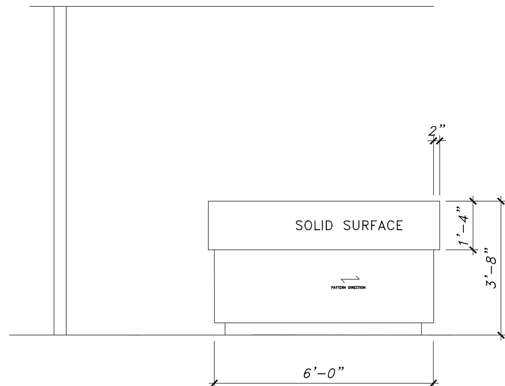
4 NURSE STATION (54) - DESK SCALE: 3/8" = 1'-0"
