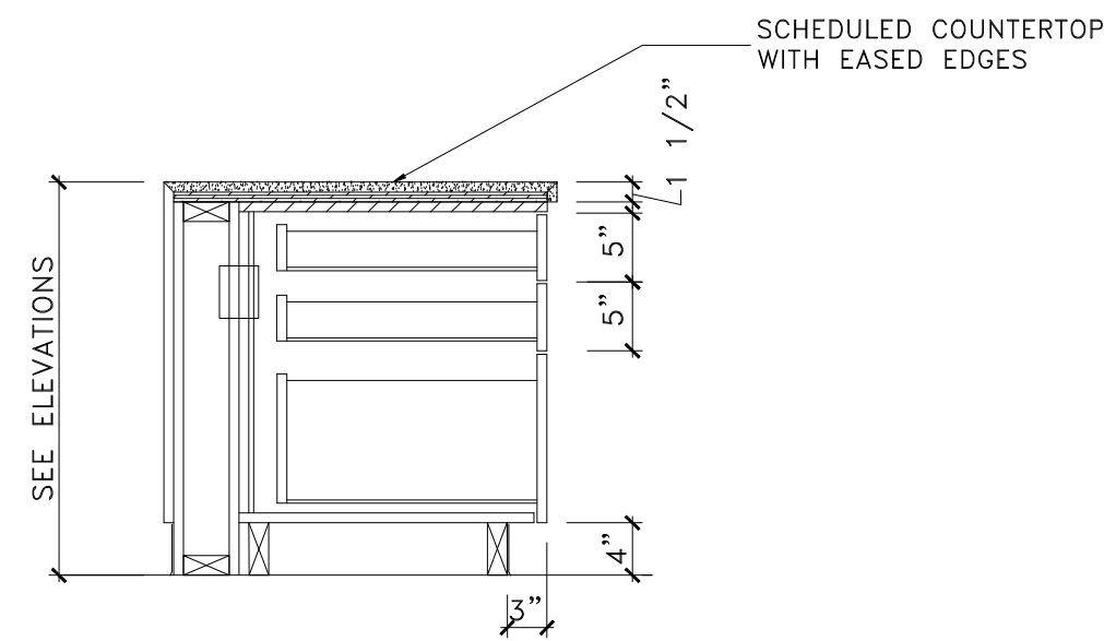
5 Rec Desk - Drawers SCALE: 3/4" = 1'-0"
