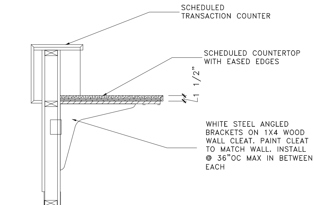
9 Nurse Desk - Open Knee Space SCALE: 3/4" = 1'-0"
