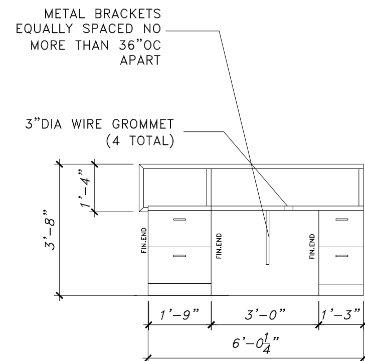
5 NURSE STATION (100, 106) - DESK SCALE: 3/8" = 1'-0"
