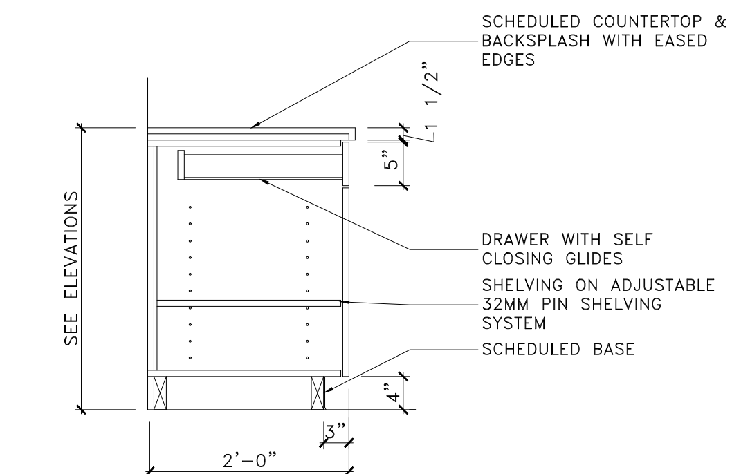
1 Base Cabinet - Drawer & Door SCALE: 3/4" = 1'-0"
