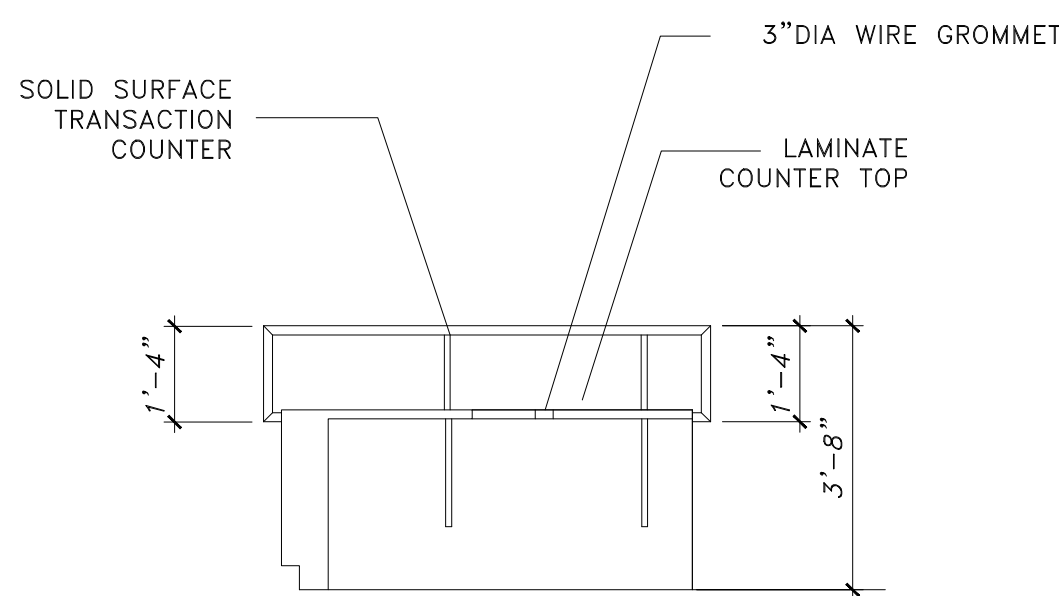
6 NURSE STATION (54) - DESK SCALE: 3/8" = 1'-0"
