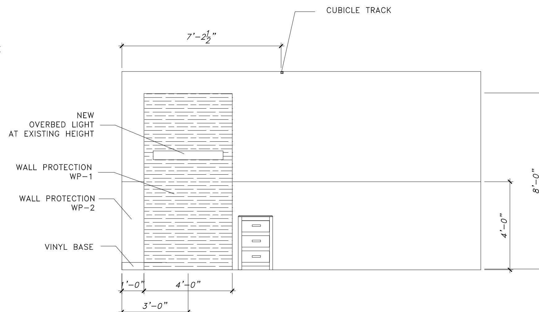
8 EAST HALL - SEMI-PRIVATE ROOM TYP. SCALE: 3/8" = 1'-0"
