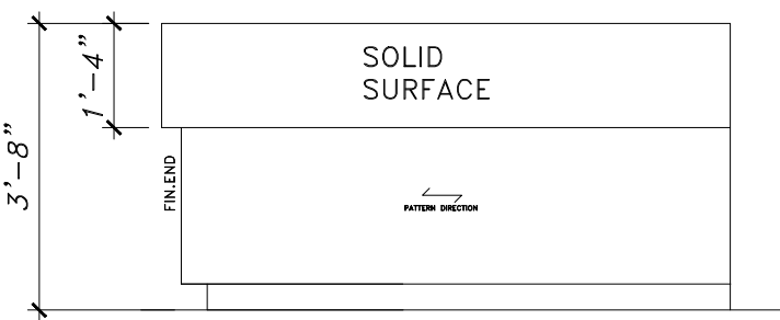
1 NURSE STATION (100, 106) - DESK SCALE: 3/8" = 1'-0"
