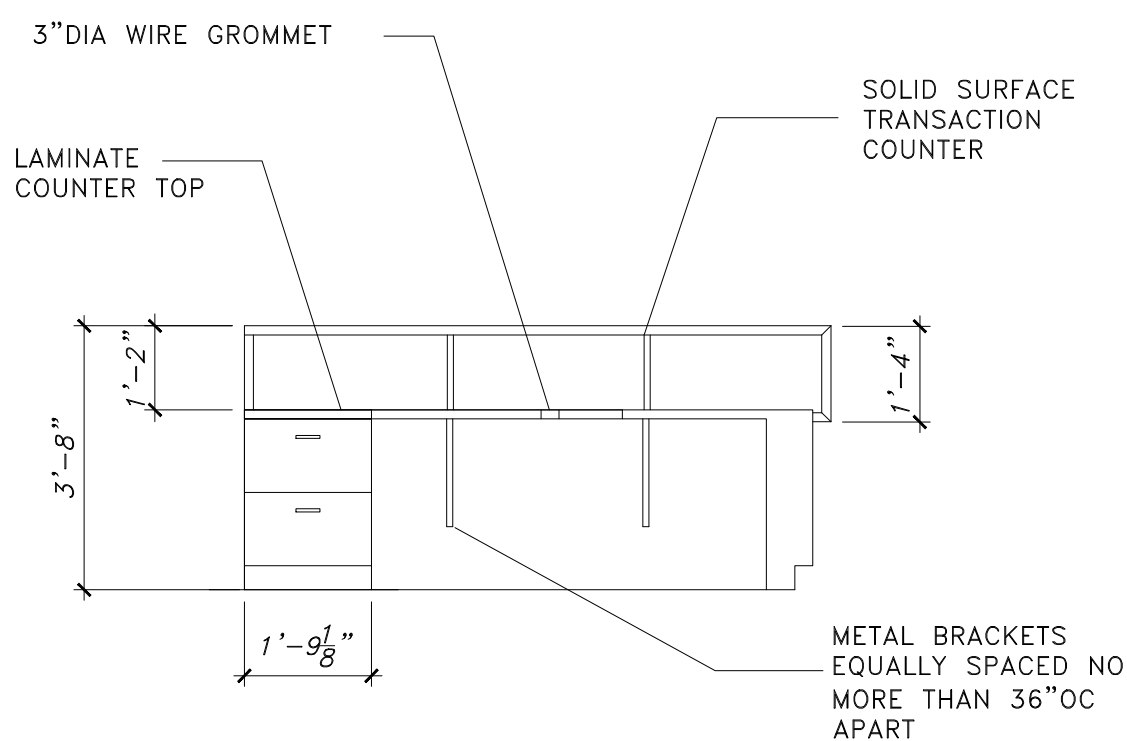
5 NURSE STATION (54) - DESK SCALE: 3/8" = 1'-0"
