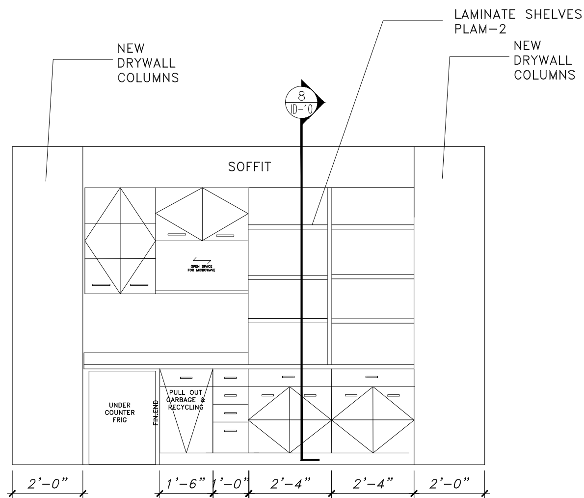
1 SPEECH THERAPY (23) - CABINETRY SCALE: 3/8" = 1'-0"
