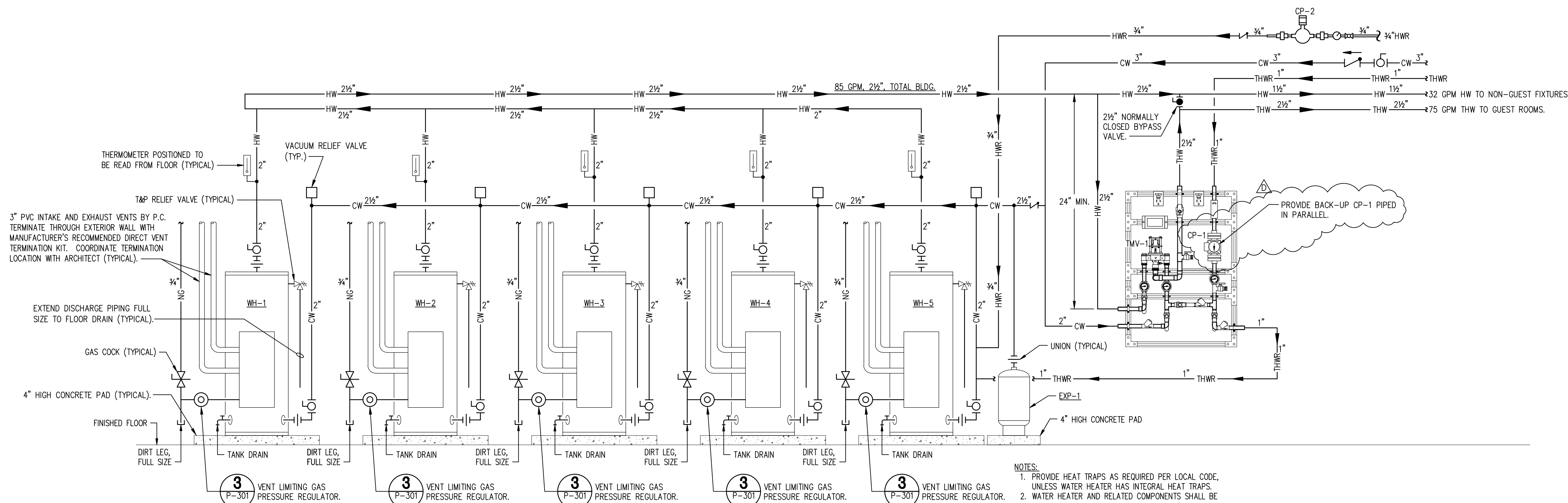
WH-1, WH-2, WH-3, WH-4, WH-5 GAS WATER HEATER SCHEMATIC 2 P-301 SCALE: NONE
