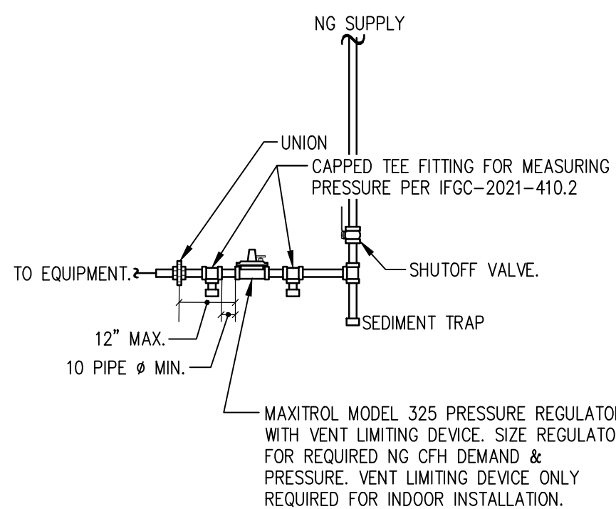
3 TYP. GAS PRESSURE REGULATOR DETAIL P-301 SCALE: NONE
