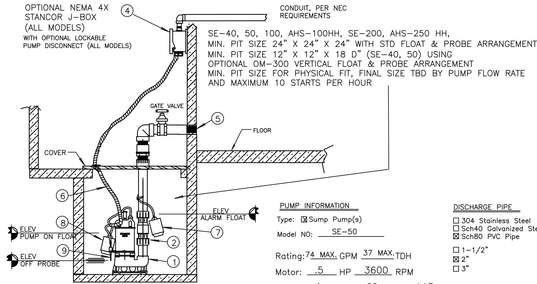
ESP ELEVATOR SUMP PUMP 1 P-301 SCALE: NONE
