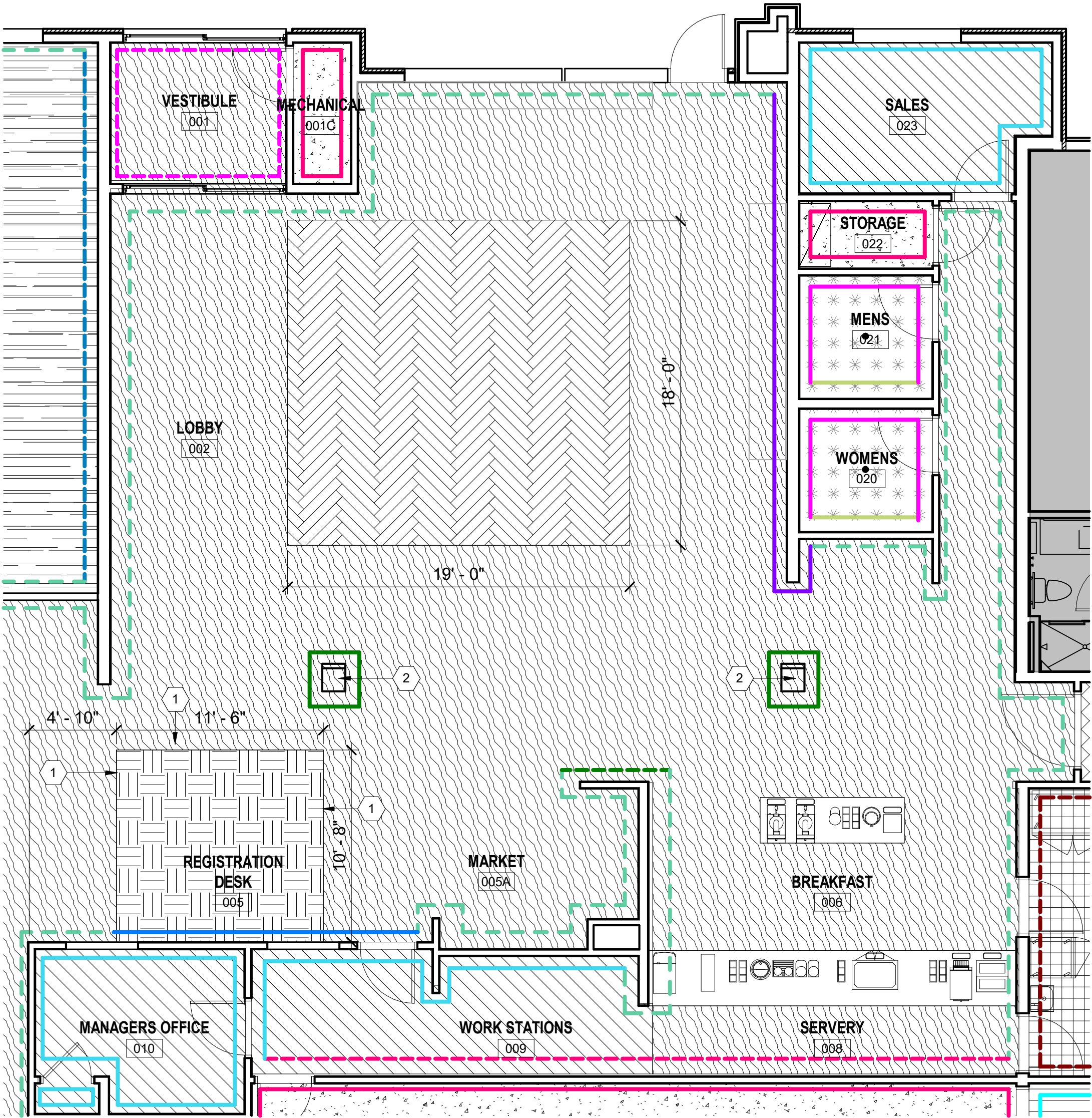
1 ENLARGED FINISH PLAN - LOBBY SCALE: 3/16" = 1'-0"
