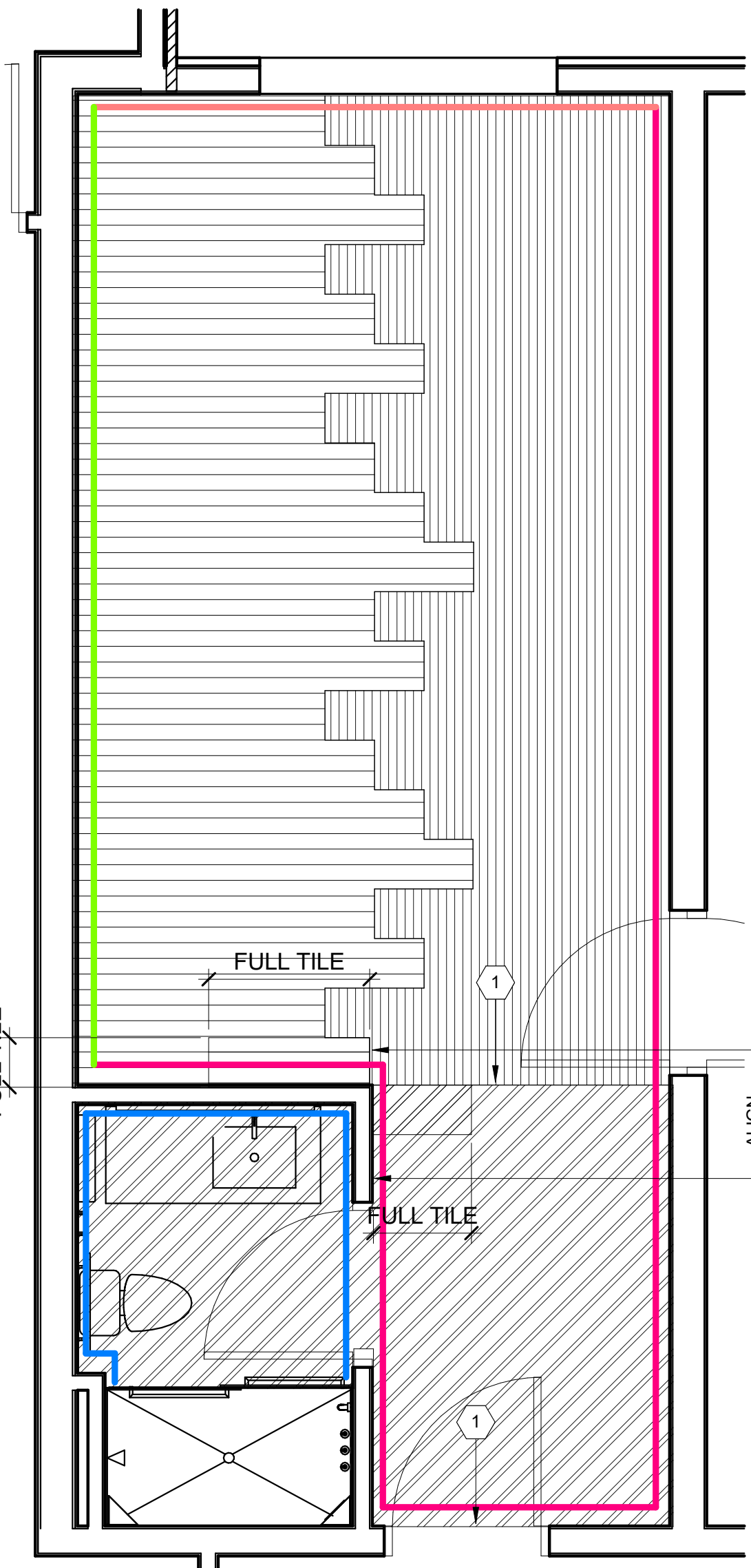
A1 KING STUDIO CONNECTOR - FINISH PLAN SCALE: 3/8" = 1'-0"
