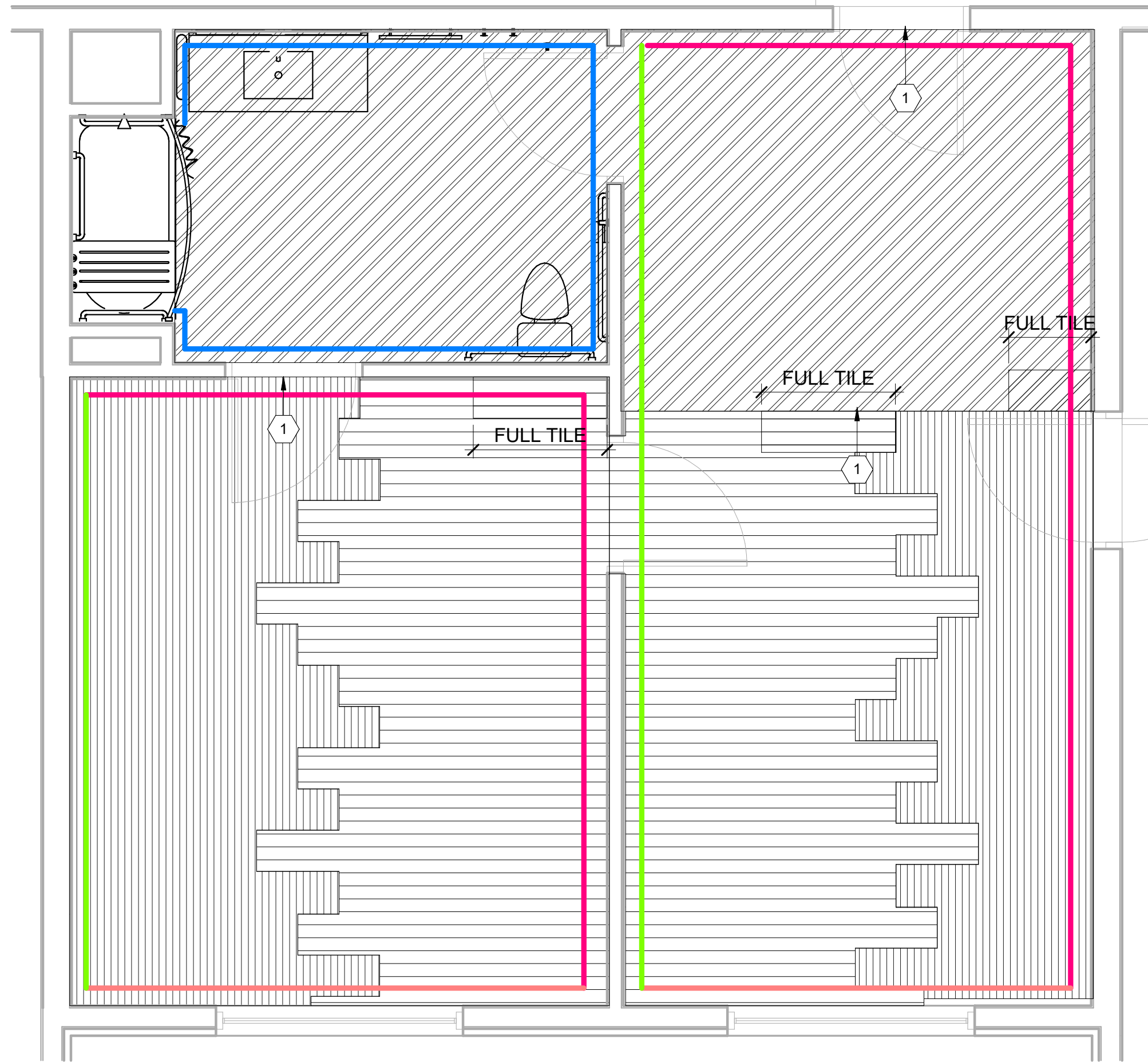
A1 KING ONE BEDROOM ACCESSIBLE - FINISH PLAN SCALE: 3/8" = 1'-0"
