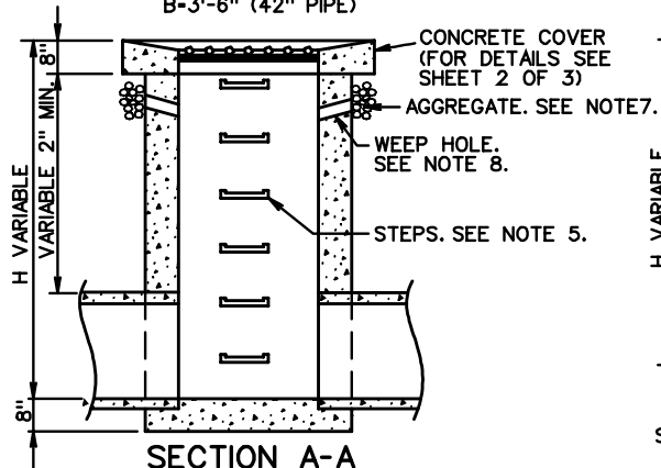
SECTION A-A CAST IN PLACE
