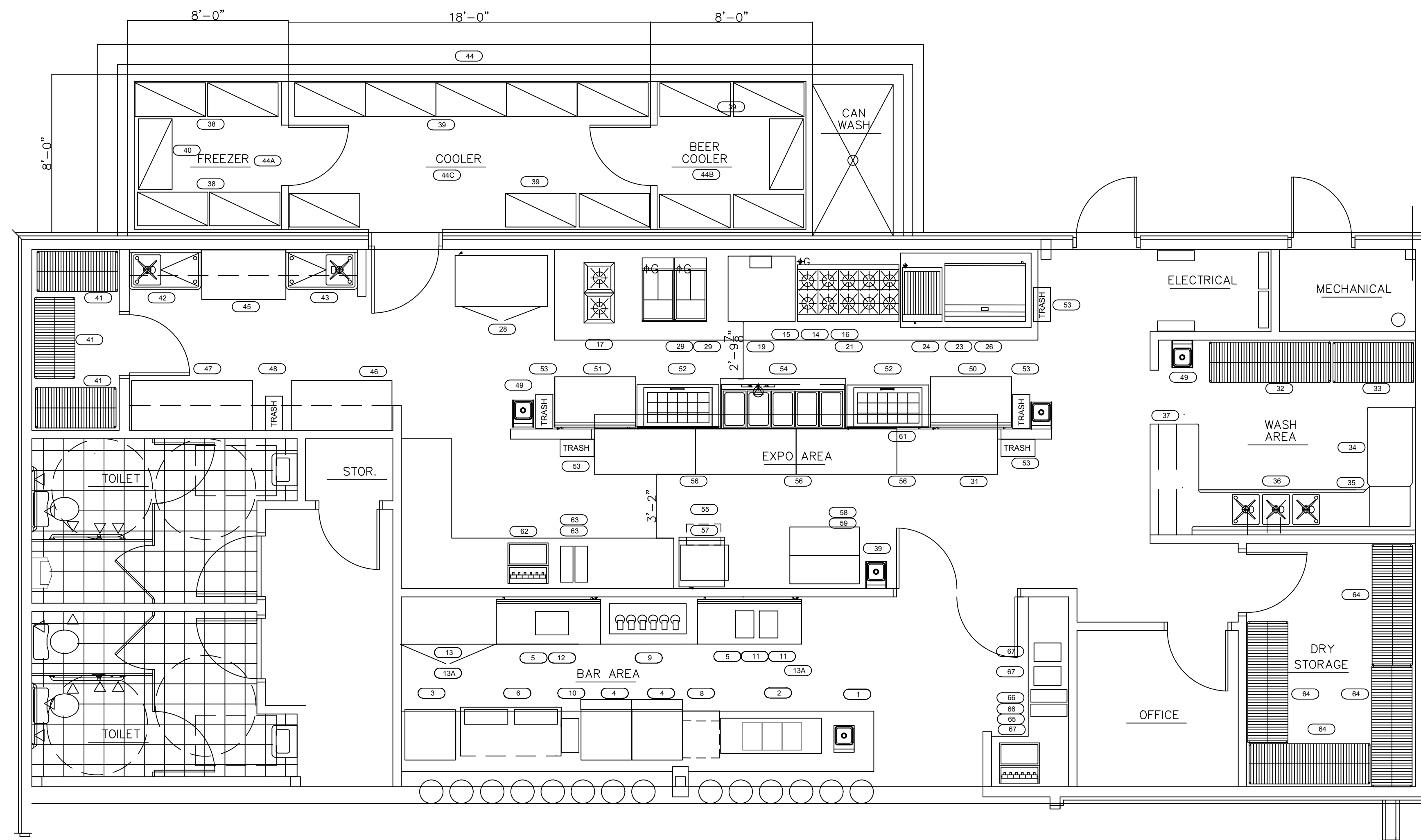
1 KITCHEN AND BAR PLAN K-1 1/4" = 1'-0"
